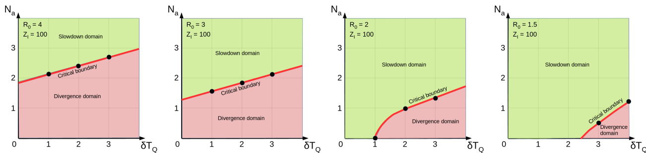
Fig. 7. Solution domains (\delta T_Q, N_a) obtained for R_0 = 4, 3, 2, 1.5 . \delta T_Q is the time-delay elapsed between the apparition of symptoms in a patient and the moment when this patient is placed in quarantine. N_a is the average number of asymptomatic persons detected and placed in quarantine when a symptomatic patient is detected. The green domains represent the models for which the epidemic spread is controlled. The red domains are the set of model for which the epidemic spread is uncontrolled with an exponential growing. The solid red lines represent the boundary between both domains and where the models are unstable with oscillations and large fluctuations.
