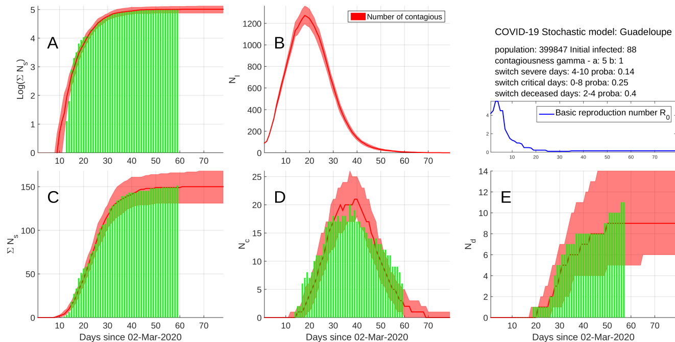
Fig. 3. Model 1 results. A) semi-logarithmic (Natural logarithm) plot of the cumulative number \Sigma N_s of severe cases. Green bars = data and red bars = model. B) Instantaneous number N_I of infectious. C) same as (A) in linear axis. D) Instantaneous number N_c of critical cases. Green bars = data and red bars = model. E) Cumulative number \Sigma N_d of deceased patients. Green bars = data and red bars = model. The parameter values used in the model are shown in the upper-right part of the figure together with the time-variation of the basic reproductive number R_0 . The red rectangles represent the 80% confidence interval centred on the median.
