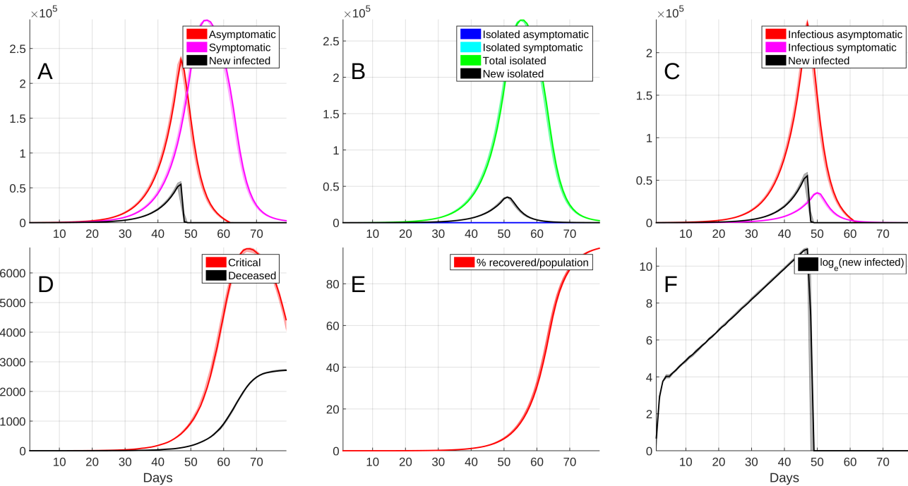
Fig. 4. Example of diverging solution obtained for R_0 = 4 , \delta T_Q = 1 day and N_a = 0 . The curves represent the median of 40 runs of the model with the same initial conditions. A) Instantaneous number of asymptomatic ( N_a ), symptomatic ( N_s ) and newly infected ( N_I ) people. B) Instantaneous number of isolated asymptomatic and newly isolated patients. In this example, no asymptomatic persons are isolated and the total number of isolated people equals the number of isolated symptomatic. C) Instantaneous number of non-isolated (i.e. infectious) symptomatic and asymptomatic people. Also shown is the number of newly infected person (also shown in A). D) Instantaneous number of patients in critical state and cumulative number of deceased patients. E) Percentage of the population infected. F) Semi logarithmic plot of the number of newly infected people (also shown in A and C with linear axes). The origin of the time axis corresponds to the beginning of the post-containment period.
