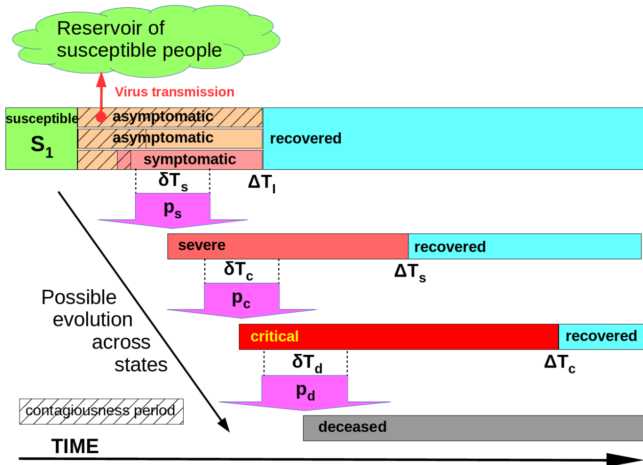
Fig. 2. Flowchart of the stochastic modelling procedure for the model proposed by Allali et al. including the detailed asymptomatic/symptomatic sequence of Figure 1. In this modified version of the model, a symptomatic patient may evolve toward the "severe" state, the "critical" state and the "deceased" state with respective probability p_s , p_c and p_d . The transition from one state to the next may only occur within time windows noted \delta T_s , \delta T_c and \delta T_d . The recovery time represents the duration after which a patient in a given state is declared "recovered", they are noted \Delta T_I , \Delta T_s and \Delta T_c respectively for the states "symptomatic and asymptomatic", "severe" and "critical".
