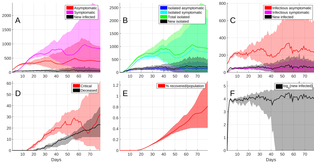
Fig. 6. Example of critical solution obtained for R_0 = 4 , \delta T_Q = 2 days and N_a = 2.3 . The origin of the time axis corresponds to the beginning of the post-containment period.
