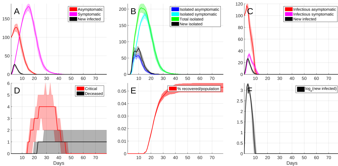
Fig. 5. Example of slow-down solution obtained for R_0 = 2 , \delta T_Q = 2 days and N_a = 3 . The coloured areas represent the envelopes of the 50% of models centred on the median model corresponding to the solid curves. The origin of the time axis corresponds to the beginning of the post-containment period.
