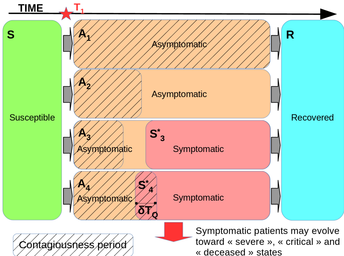
Fig. 1. Flowchart of the possible evolution schemes for the "asymptomatic" and "symptomatic" classes of the model. At time T_1 , 4 susceptible persons are infected. At the beginning, all four patients are asymptomatic (orange areas) and contagious (hatched areas). When becoming symptomatic (red areas), patient S_4 is identified, tested and isolated. The \delta T_Q parameter represents the time-delay elapsed between the apparitions of the symptoms and the moment when the patient is placed in quarantine to suppress her/his contagiousness. This marks the end of her/his contagiousness period. Asymptomatic patients (e.g. A_3 and A_2 located in the entourage of S_4 ) are tested and isolated. Patient A_1 remains asymptomatic and undetected all along her/his illness period. In the model, patients S_3 and S_4 may evolve to other states: "severe", "critical" and "deceased" (see (1) for details).
