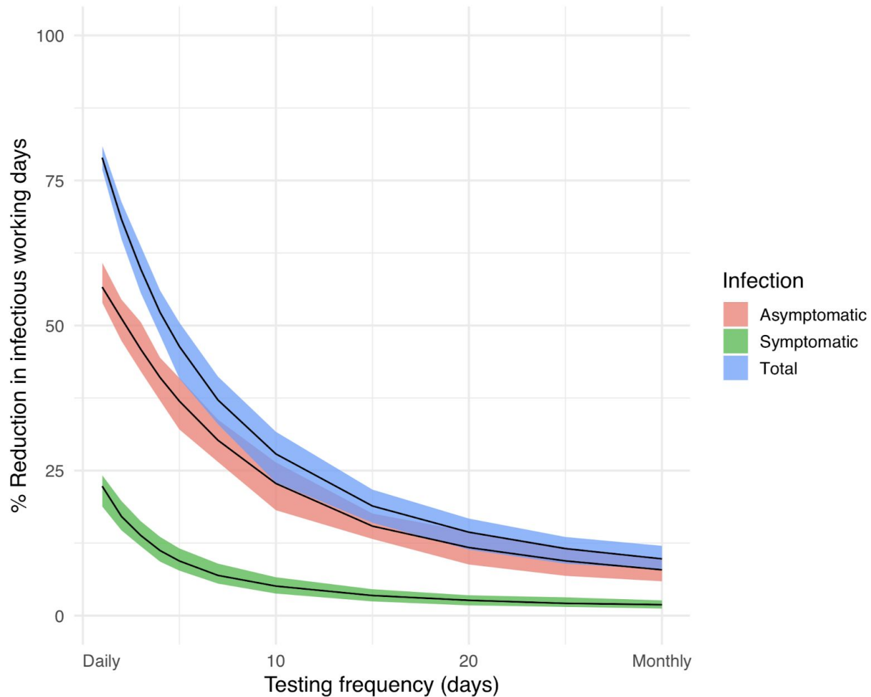
Figure 1: Projected effectiveness of routine PCR testing frequency on reduction on transmission for high risk workers, assuming the proportion of asymptomatic cases is 40% with the R_0=3 . Error bars represent the minimum and maximum bounds of projected reduction, varying sensitivity and specificity of the PCR test and assumptions on natural history of transmission.
