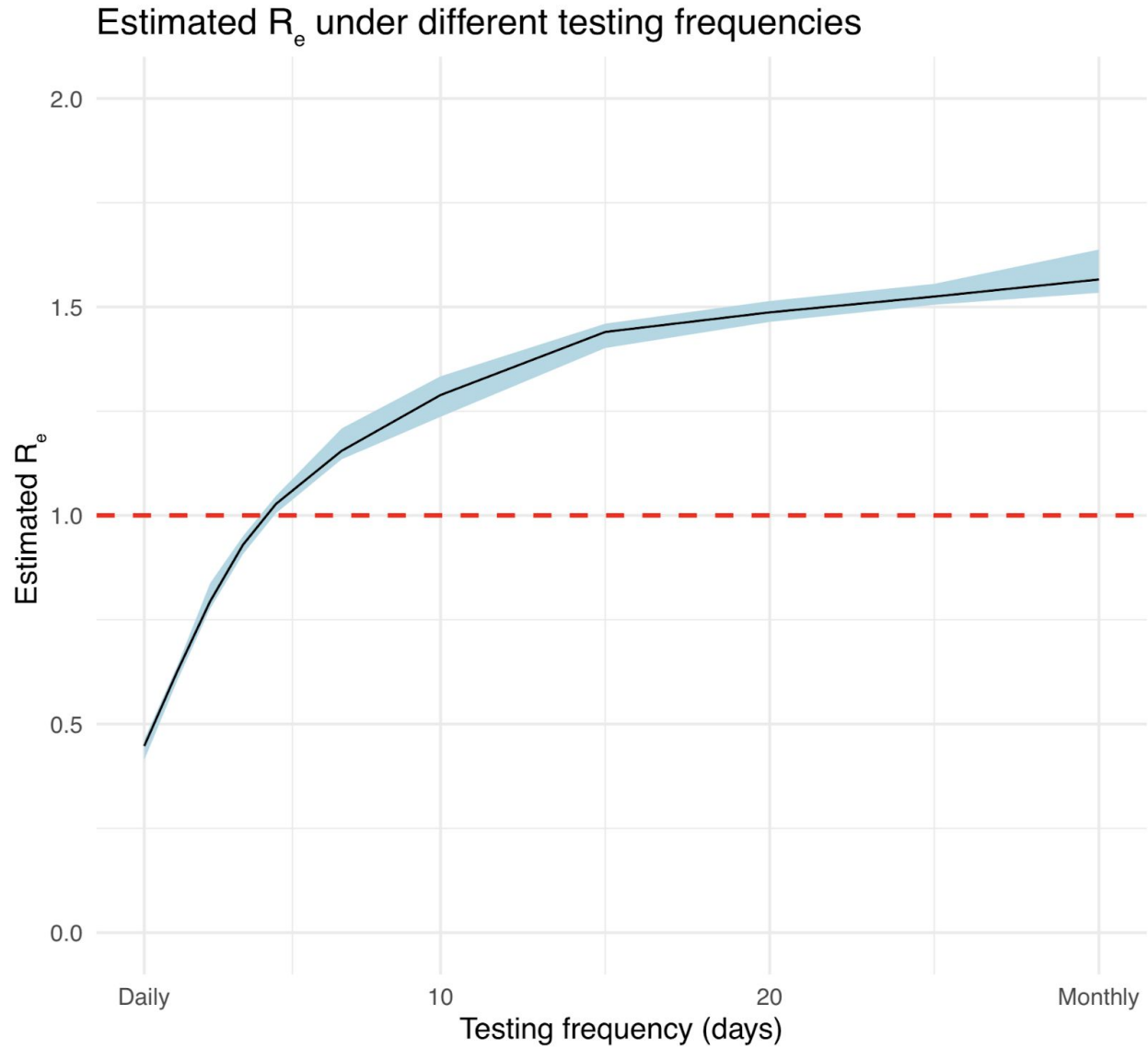
Figure 2: Projected effective reproduction number ( R_e ) in a susceptible workplace. Bounds represent the estimated minimum and maximum values.
