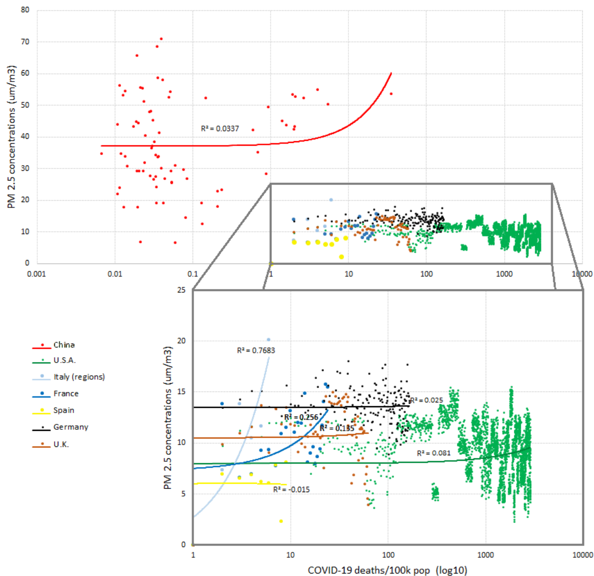
Graph 1 - Correlational plots of COVID-19 fatalities with the satellite-based PM 2.5 concentrations for seven countries except the missing fatalities of Iran. The countries should not be compared in respect to mortality rate due to different administration sizes.
