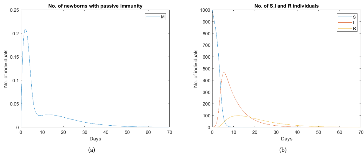
Figure 3: MSIR Model
