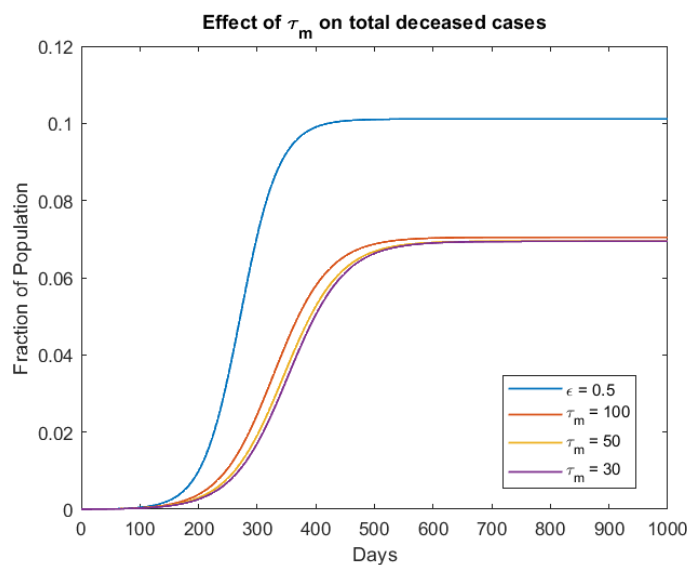
Figure 16: Effect of total deceased cases: D
