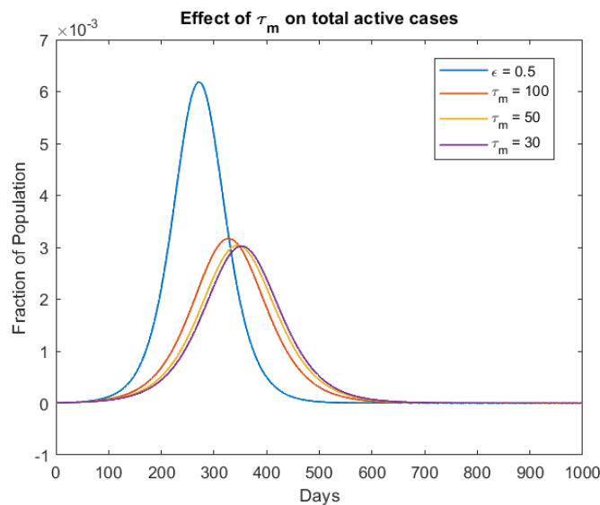
Figure 15: Effect on the total active cases: I_s + I_{as} + Q + Q' + C
