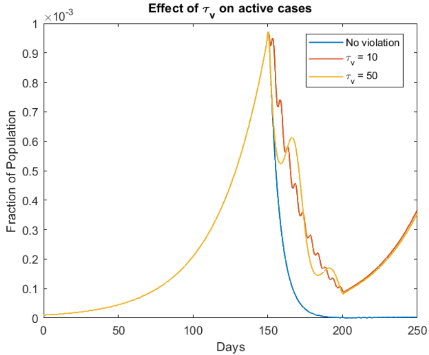
Figure 13: A zoomed picture of the above plot for t < 250
