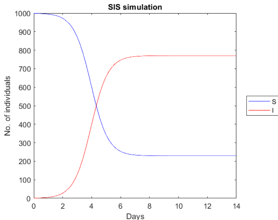
Figure 2: \alpha = 2.18 , N = 1000 , \beta = 0.5 , S(0) = 999 , I(0) = 1
