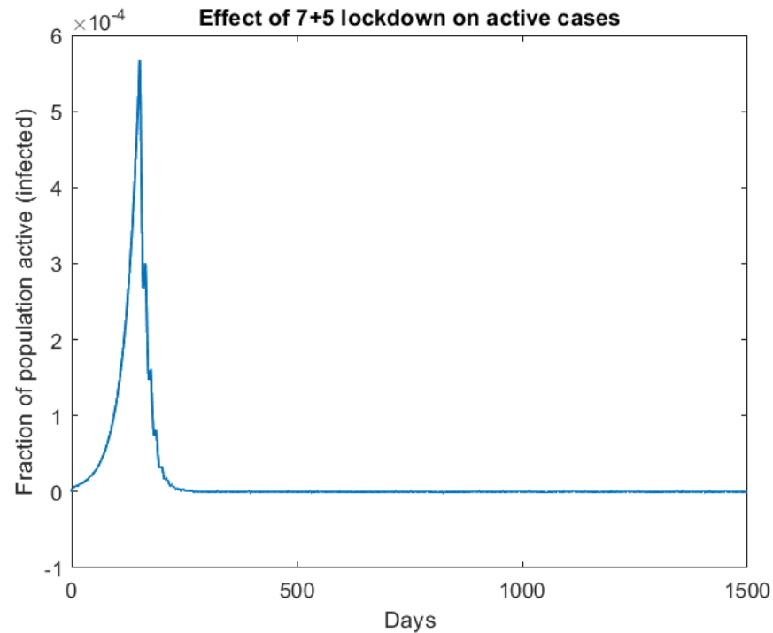
Figure 9: 7+5 lock down from 150 days to eternity
