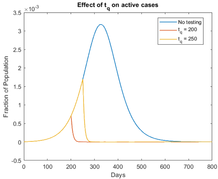
Figure 19: Effect on the total active cases: I_s + I_{as} + Q + C for \tau_q = 250
