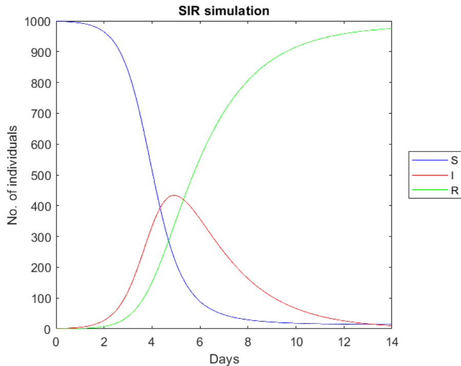
Figure 1: \alpha = 2.18 , N = 1000 , \beta = 0.5 , S(0) = 999 , I(0) = 1 , R(0) = 0
