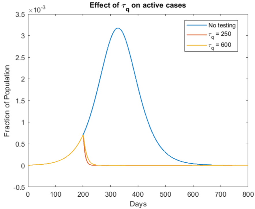
Figure 17: Effect on the total active cases: I_s + I_{as} + Q + C for t_q = 200
