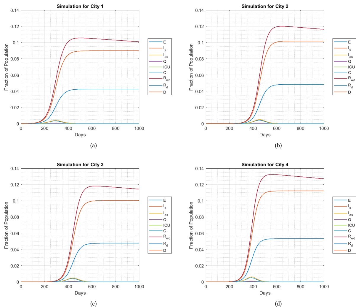
Figure 20: Patient zero belongs to City1
