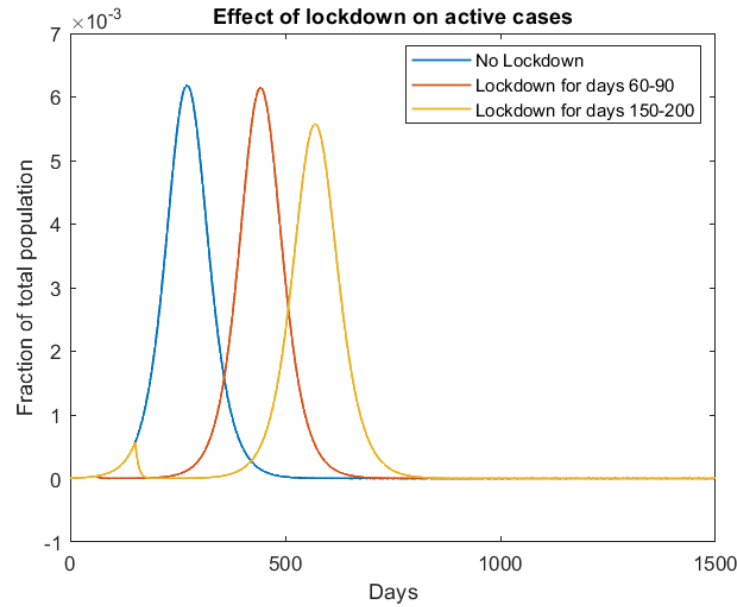
Figure 6: Effect on net active cases: I_s + I_{as} + Q + Q' + C
