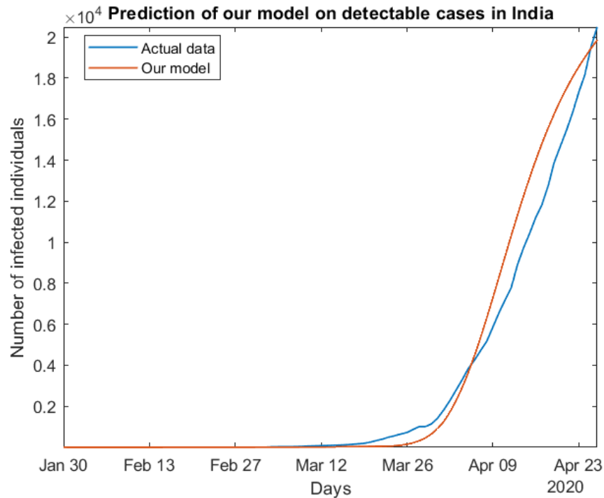
Figure 22: Comparison with actual data. N(0) = 1399999964 , E(0) = 25 , I'_s(0) = 2 , I_s(0) = 0 ; I_{as}(0) = 2 , Q(0) = 2 , rest = 0
