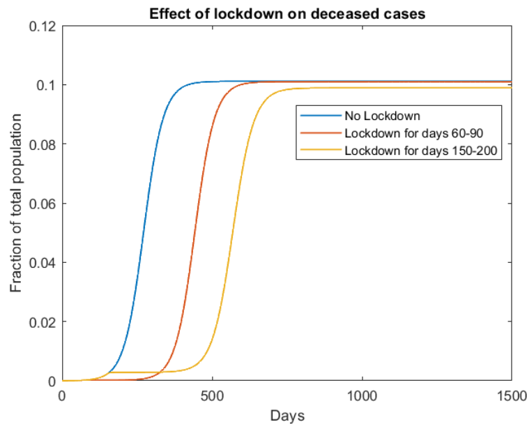
Figure 7: Effect on D compartment
