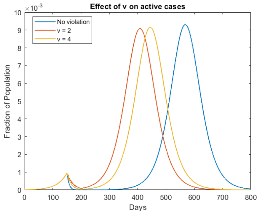
Figure 14: Effect on the total active cases: I_s + I_{as} + Q + Q' + C for \tau_v = 10
