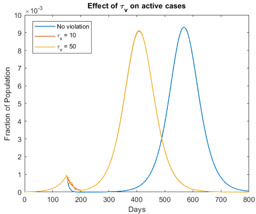
Figure 12: Effect on the total active cases: I_s + I_{as} + Q + C for v = 2
