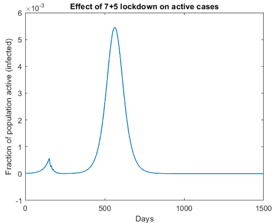
Figure 10: 7+5 lock down for 150-250 days
