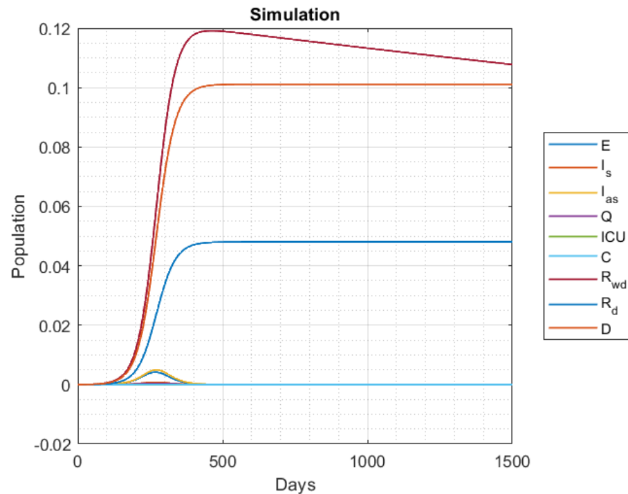
Figure 5: Initial conditions: S(0) = 1 - 1 \times 10^{-5} , E(0) = 1 \times 10^{-5} , others = 0
