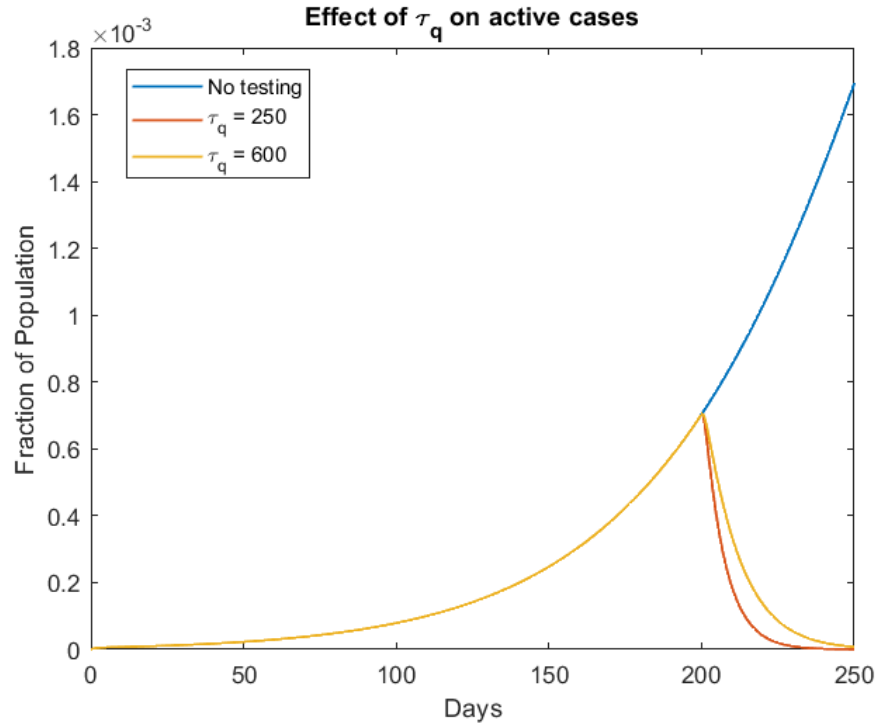
Figure 18: A zoomed picture of the above plot for t < 250
