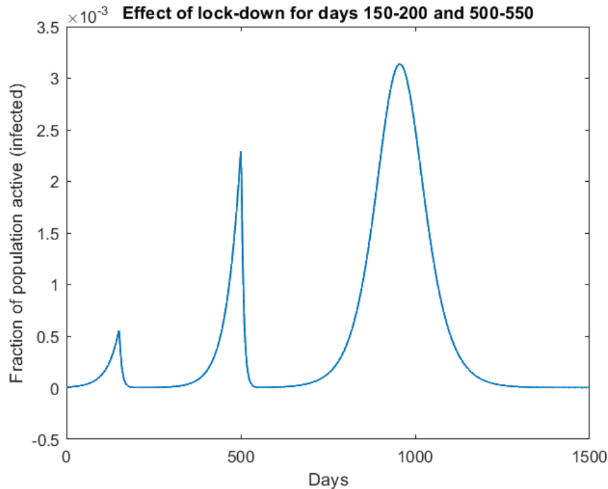
Figure 8: lock down for both days 150-200 and 500-550
