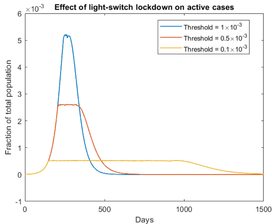
Figure 11: Effect of light-switch lock down on active cases
