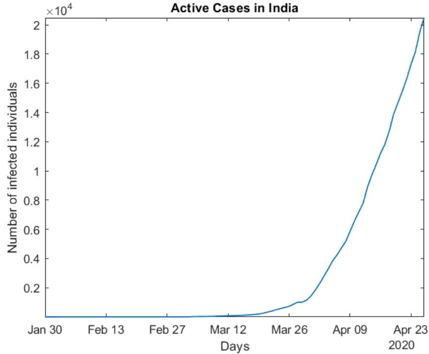
Figure 21: Active Cases timeline of India
