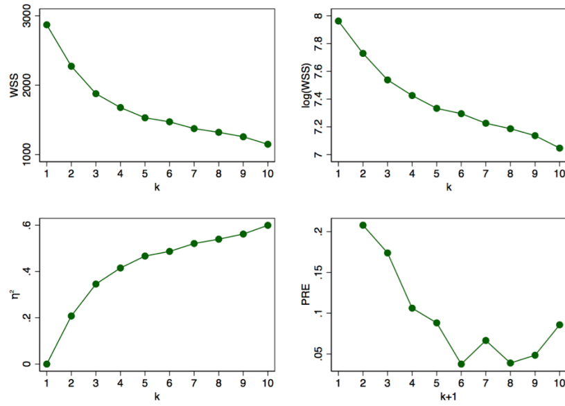
Figure 2. WSS, log(WSS), \eta^2 coefficient and PRE for 10 cluster solutions when features are standardized, Michigan, 2008-2011
