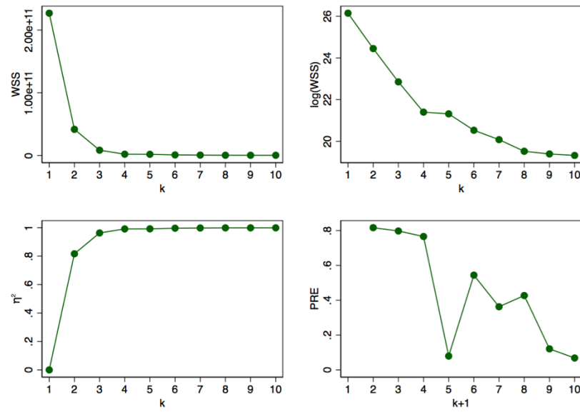
Figure 1. WSS, \log(\text{WSS}) , \eta^2 coefficient and PRE for 10 cluster solutions when features are not standardized, Michigan, 2008-2011
