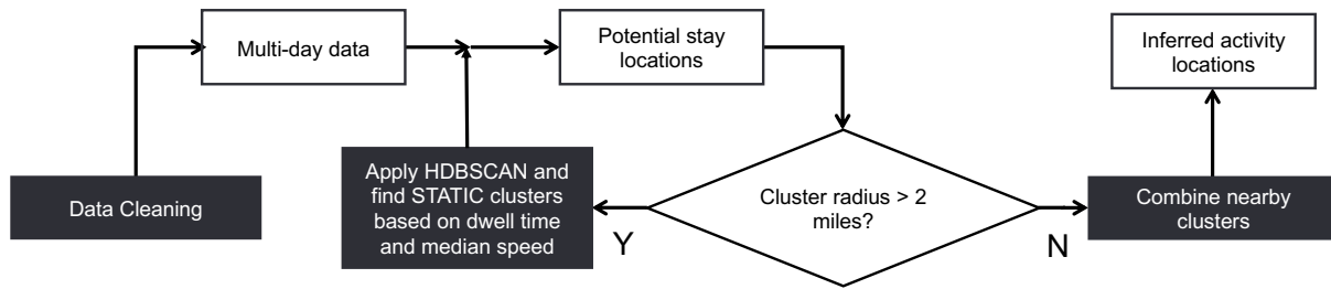
4 Figure 4. Activity clustering methodology
