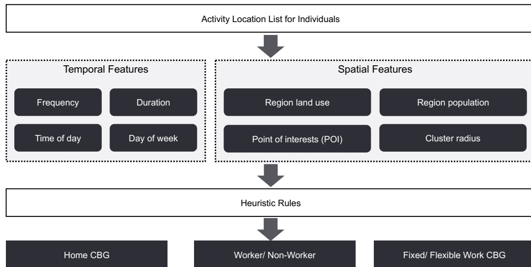
19 Figure 5. Home/work CBG imputation methodology
