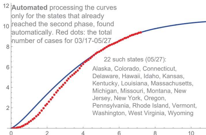
FIGURE 15. Only for the states reached 2nd stage on 05/27.
