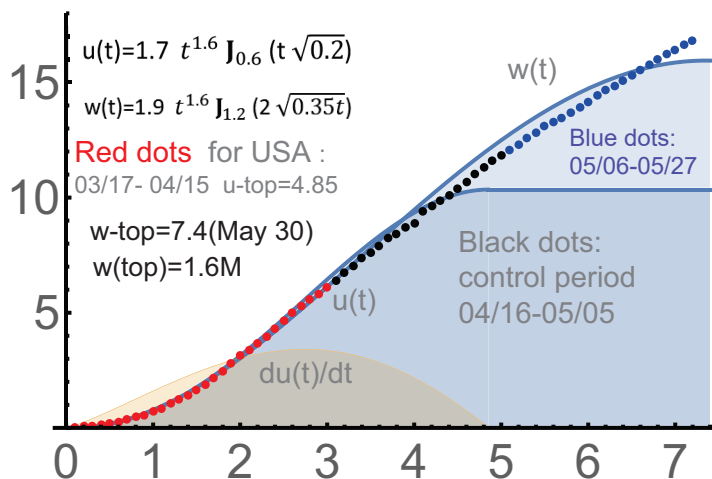
FIGURE 6. USA: c=2.2, a=0.2, C=1.7; b=0.35, D=1.9 .
