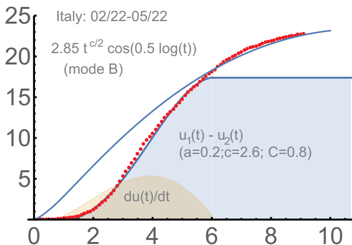
FIGURE 10. Italy: c=2.6, a=0.2, d=0.5
