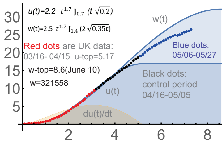
FIGURE 7. UK: c=2.4, a=0.2, C=2.2; b=0.35, D=2.5 .
