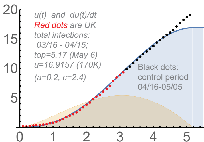
FIGURE 3. u(t) = 2.2 t^{(c+1)/2} J_{(c-1)/2}(\sqrt{at}) for c = 2.4, a = 0.2
