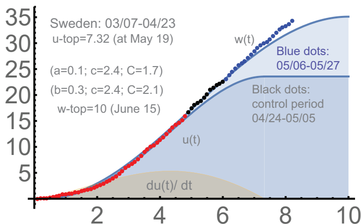
FIGURE 8. w(t) = 2.1t^{(c+1)/2} J_{c-1}(2\sqrt{bt}) ; b=0.3, c=2.4 .
