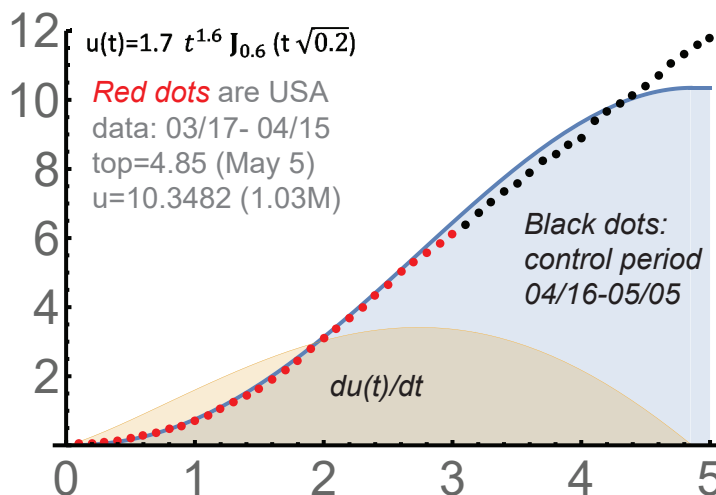
FIGURE 2. u(t) = 1.7 t^{(c+1)/2} J_{(c-1)/2}(\sqrt{at}) for c = 2.2, a = 0.2
