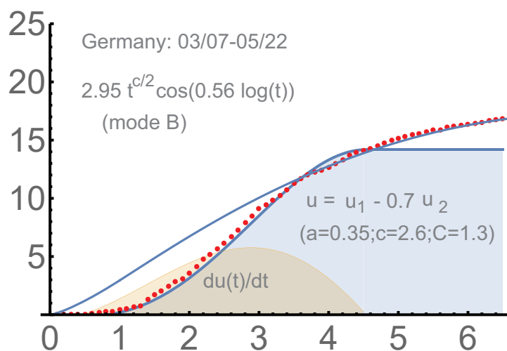
FIGURE 11. Germany: c=2.6 , a=0.35 , d=0.56
