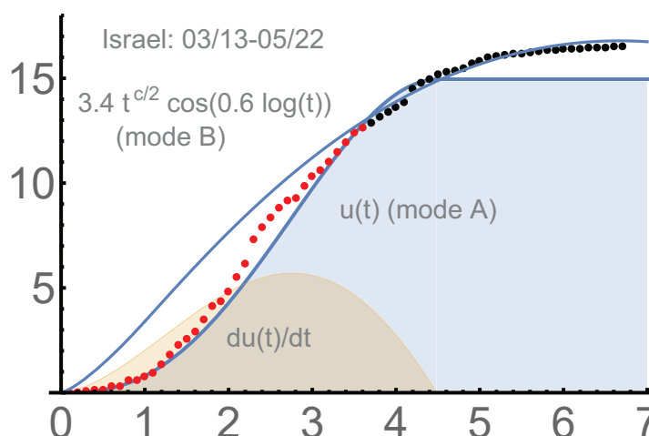
FIGURE 9. Israel: c=2.6, a=0.3, d=0.6
