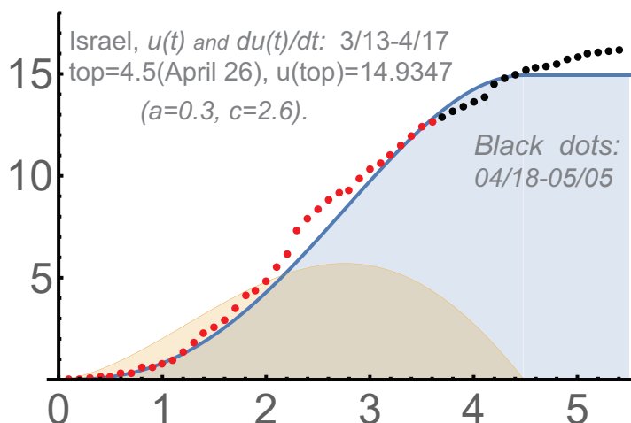
FIGURE 5. u(t) = 2.2 t^{(c+1)/2} J_{(c-1)/2}(\sqrt{at}) for c = 2.6, a = 0.3
