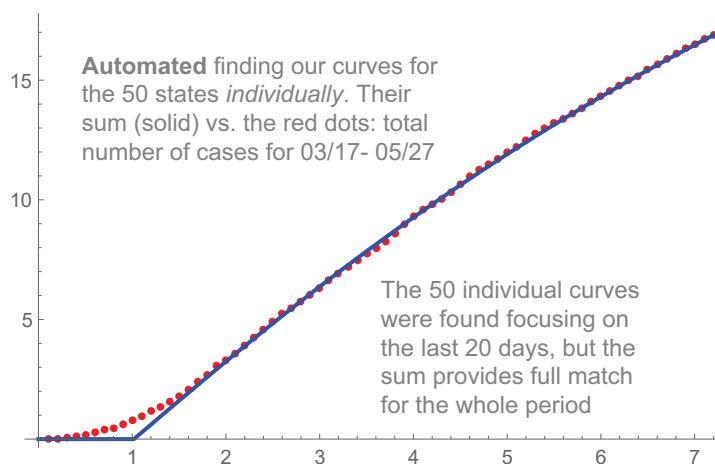
FIGURE 14. USA, the total of the curves for individual states.
