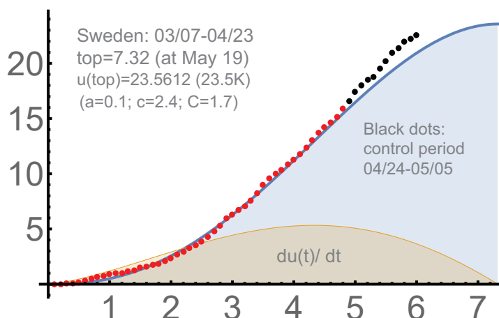
FIGURE 4. u(t) = 1.7 t^{(c+1)/2} J_{(c-1)/2}(\sqrt{at}) for c = 2.4, a = 0.1
