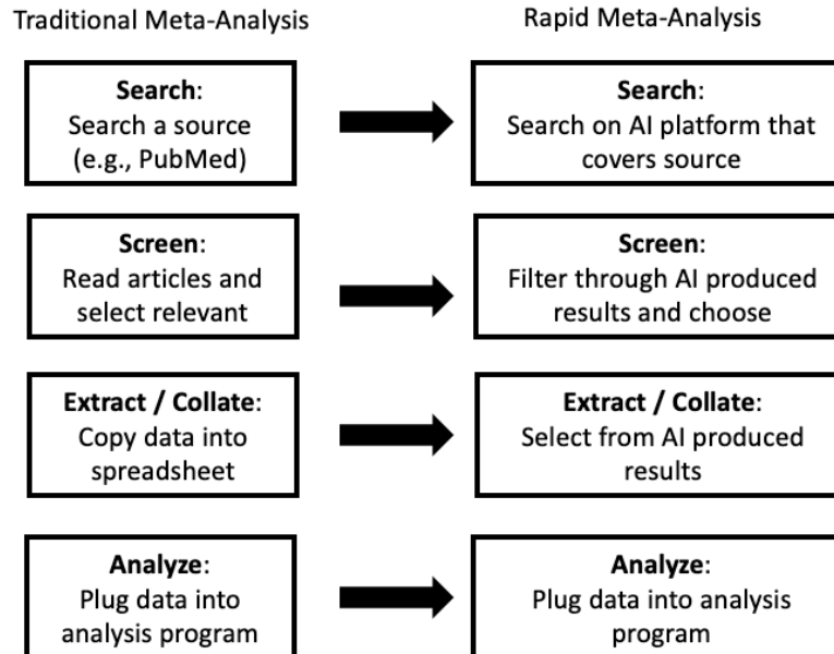
Figure 1: Traditional meta-analysis (simplified, left) vs. RMA using AI (right)
