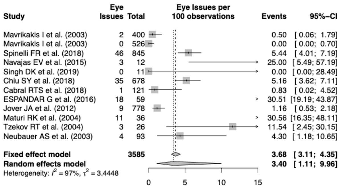
Figure 3: Forest plot for our RMA
