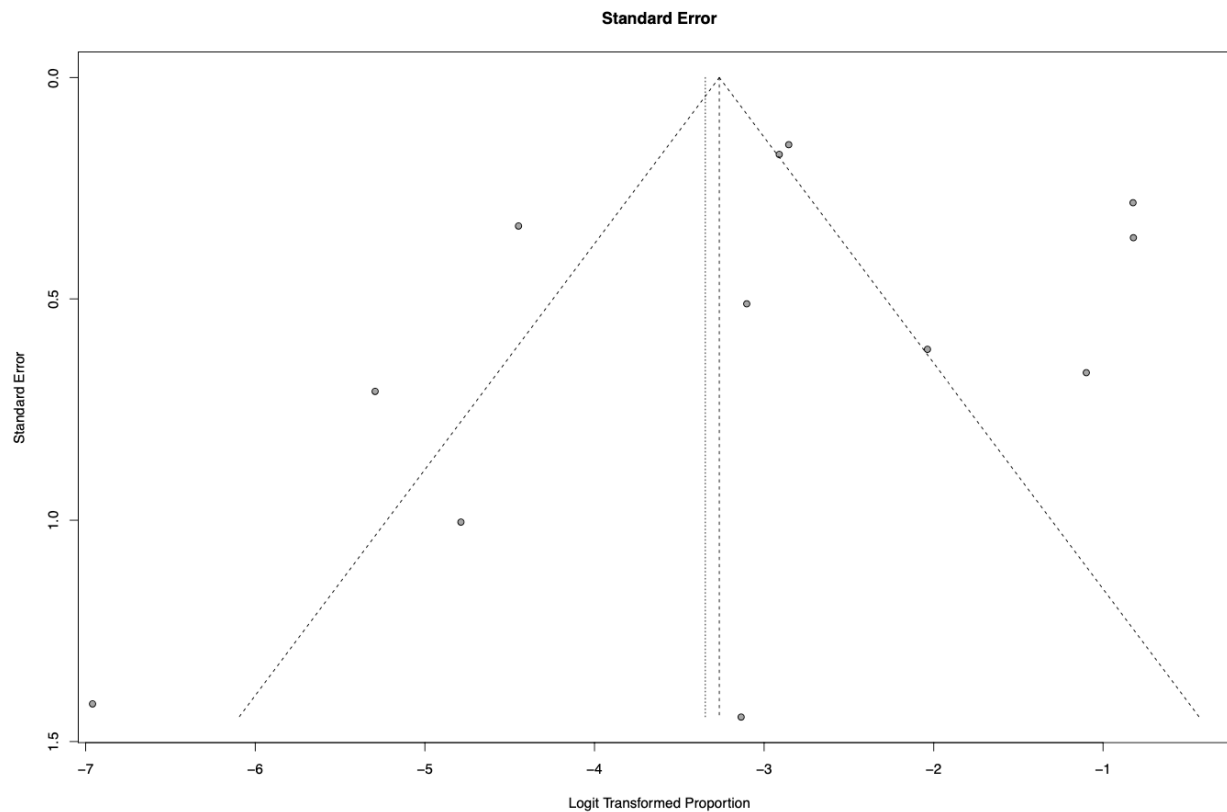
Figure 4: Funnel plot for our RMA
