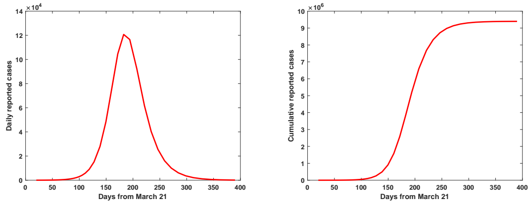
Figure 3.3: Time series plot for model (2.2), starting from March 21, 2020, with p = 0.55 . Left panel corresponds the numbers of confirmed symptomatic infectious individuals. Right panel corresponds the numbers of cumulative confirmed symptomatic infectious individuals.
