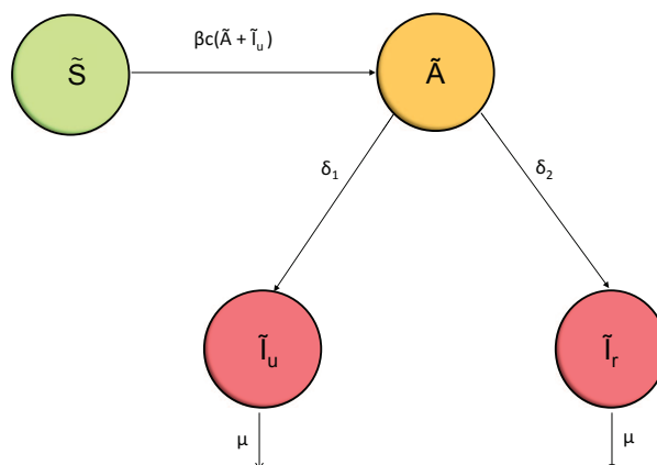
Figure 2.1: Basic 2019-nCoV transmission diagram
