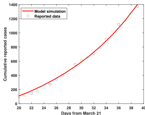
Figure 3.2: Comparison between time series of cumulative reported cases for model (2.2) with p = 0.55 and reported data of cumulative number of confirmed cases of COVID-19 from March 21 to April 9, 2020. The dots are the day by day reported data in Table 1. The red solid line is the fitting curve of model (2.2).
