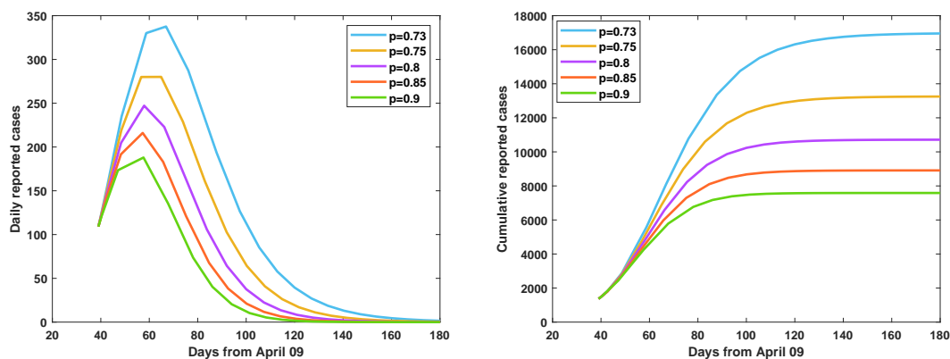
Figure 3.4: Time series plot for model (2.2), starting from April 9, 2020, of the numbers of reported individuals change using different containment rates ( p \in \{0.73, 0.75, 0.8, 0.85, 0.9\} ). Left panel corresponds the numbers of daily reported individuals. Right panel corresponds the numbers of daily cumulative reported individuals.
