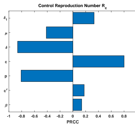
Figure 3.6: Sensitivity analysis. The partial rank correlation coefficients are shown using the control reproduction number.
