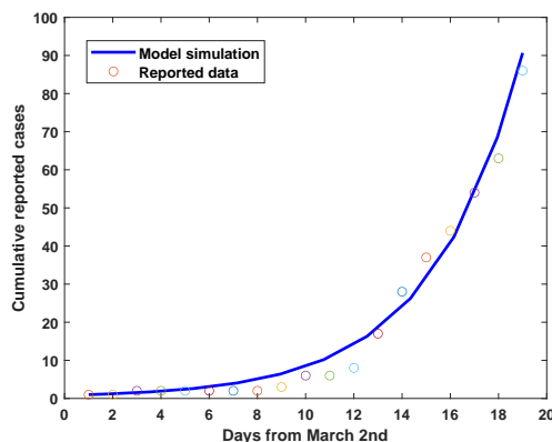
Figure 3.1: Comparison between time series of cumulative reported cases for model (2.1), with a = 0.296 and b = 0.555 , and reported data of cumulative confirmed cases of COVID-19 from March 2nd to March 20, 2020. The dots are the day by day reported data in Table 1. The blue solid line is the fitting curve of model (2.1).
