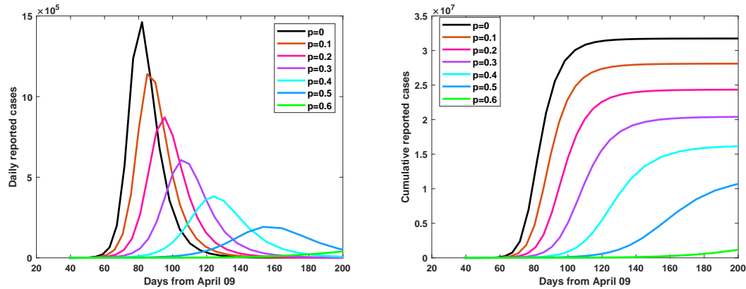
Figure 3.5: Time series plot for model (2.2), starting from April 9, 2020, of the numbers of reported individuals change using different containment rates ( p \in \{0.1, 0.2, 0.3, 0.4, 0.5, 0.6\} ). Left panel corresponds the numbers of daily reported individuals. Right panel corresponds the numbers of daily cumulative reported individuals.
