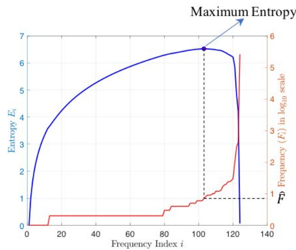
Figure 6: Entropy of the unique states. We see that as we adding states with low frequency, the entropy increase. However, at some point where the frequency of the state is significantly larger than previous frequency, the entropy decrease. The point of maximum entropy can be seen as a critical point, and the states before and after this point have different information and belong to different categories.
