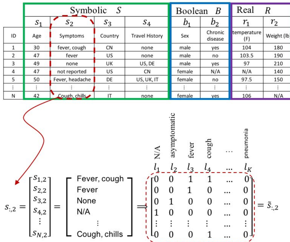
Figure 3: Booleanization of non-Boolean variables illustrative example. By this example, we illustrate how to convert standard descriptive variables, such as the commonly named symptoms, into a Boolean matrix as this is a required initial stage for our analysis. See Eqs. (1)-(3).
