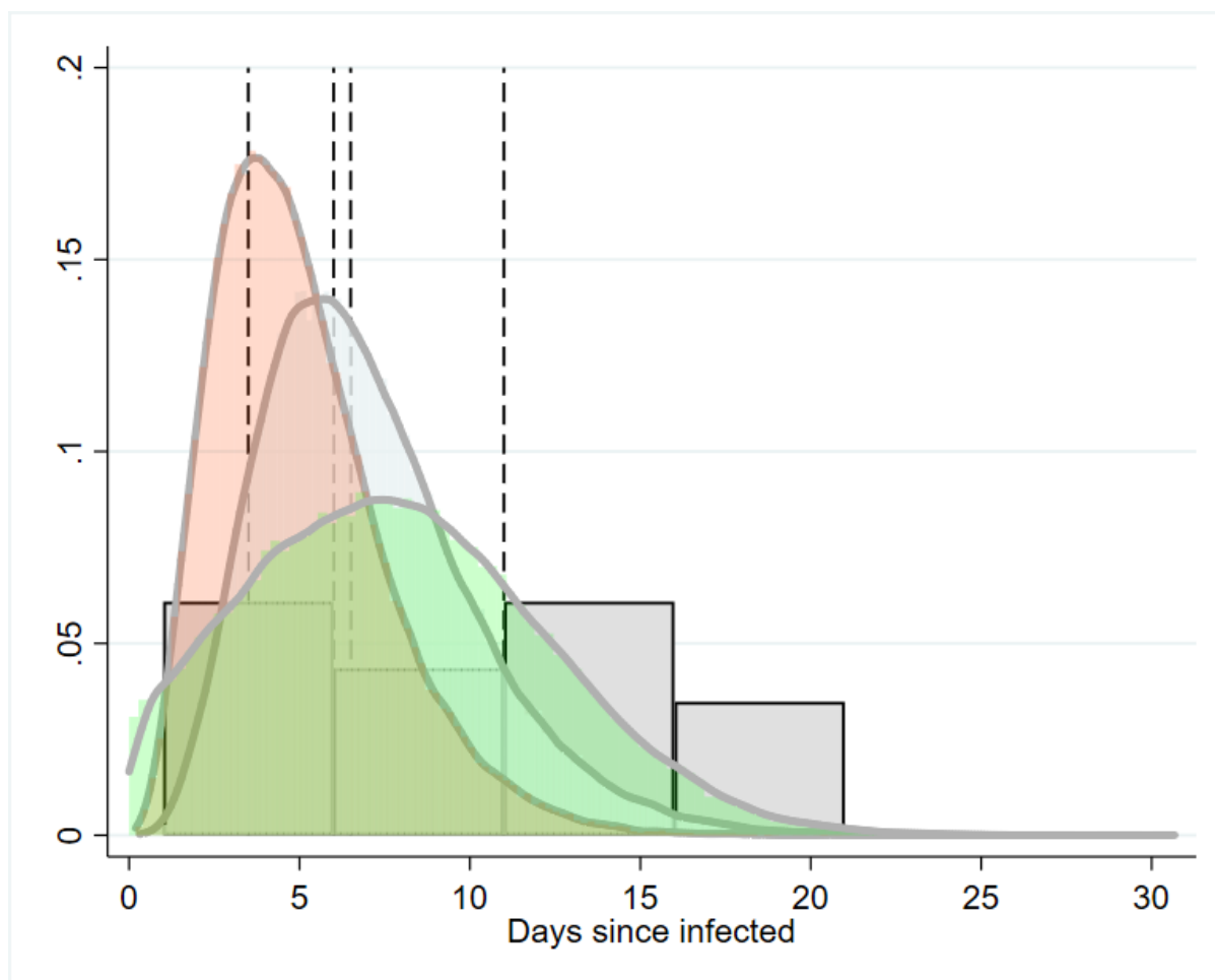
734 Figure 1: Simulation of the parameter distribution inferred for duration infectious period for 735 asymptomatic cases (T2) inferred infectious period for Davies et al. (2020a), grey/blue curve, Davies 736 et al. (2020b) pink curve [model priors]. Green curve: Ma et al. (2020). Histogram is the distribution 737 of asymptomatic cases to two clear tests reported by Hu et al. (2020). Reference lines are point 738 estimates reported from Zhou et al. (2020), Li et al. (2020), and Tuite et al. (2020a & 739 b).[7,8,14,15,26,27,39,71]
