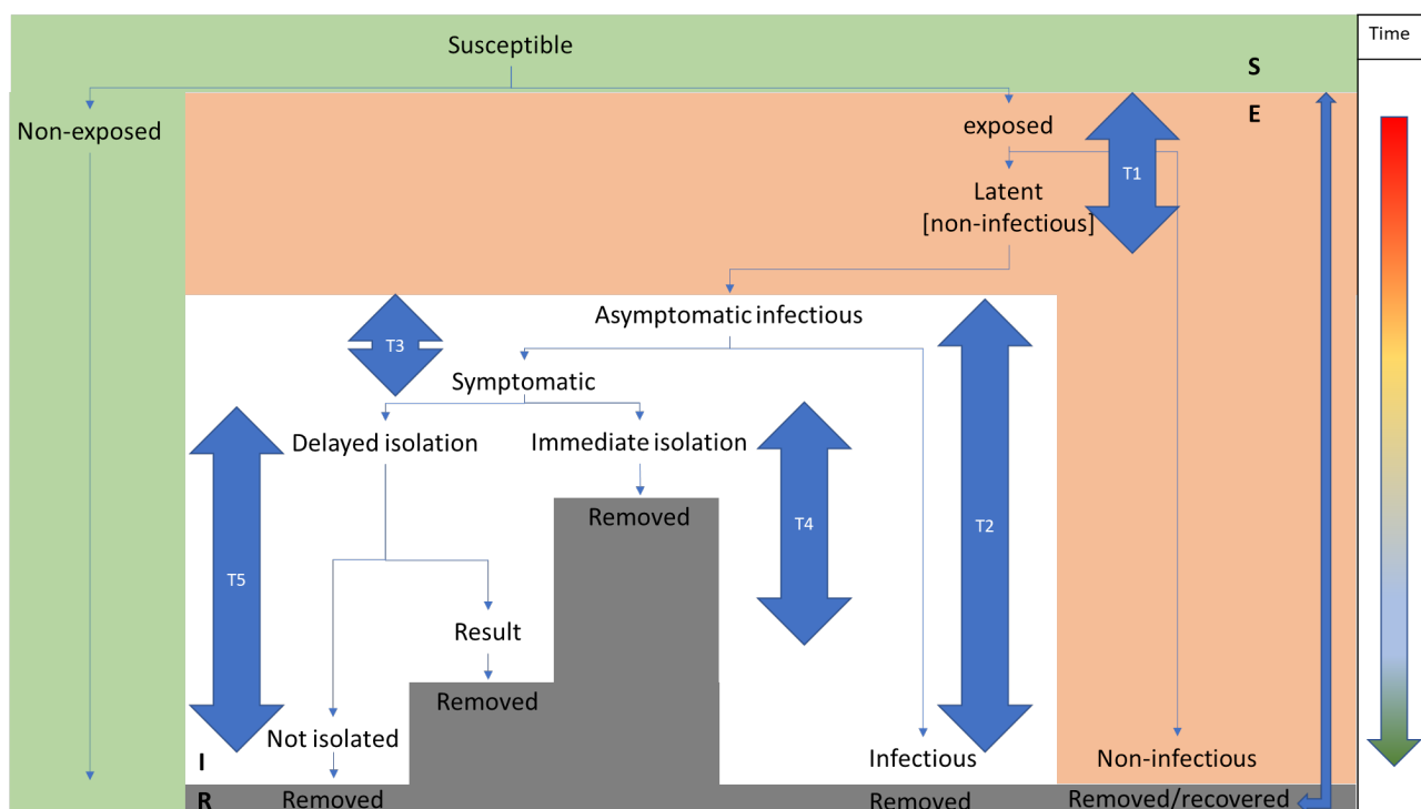
797 Figure S1: Conceptual model of the key temporal parameters impacting COVID-19 infection 798 progression over time. T1: Latent period; T2: Asymptomatic infectious period; T3: Pre-symptomatic 799 infectious period; T4: Symptom onset to diagnosis [self-isolation] or hospitalisation; T5: Symptom 800 onset to removed [death or recovery]
