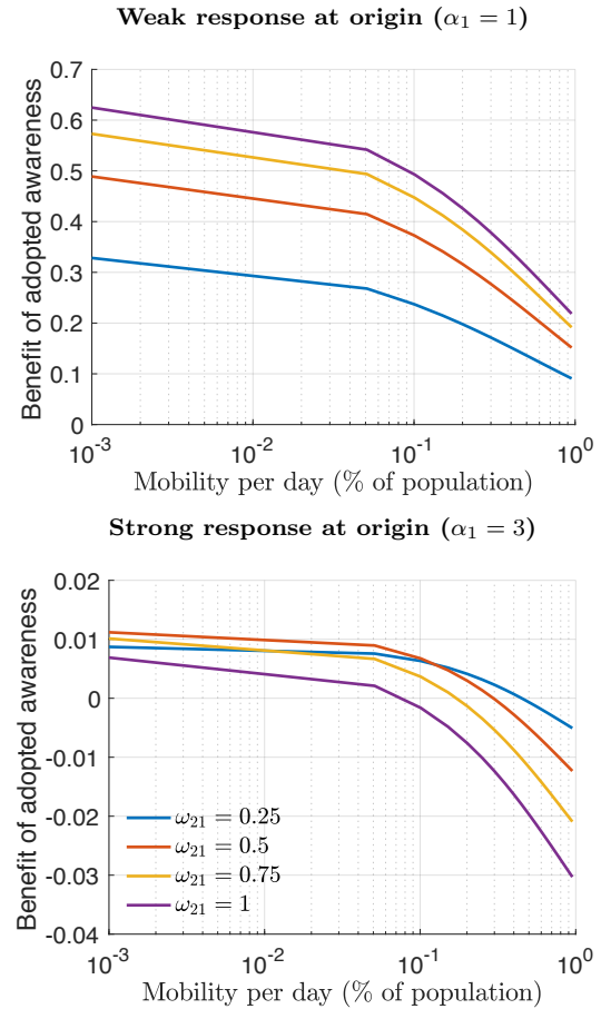
Figure 6: Benefit of adopted awareness with respect to mobility rates. (Top) Weak and (Bottom) strong responses at the origin. The strength of response at Locality 2 is weak \alpha_2 = 1 . The benefit is measured as the reduction in final size with respect to the zero-adopted awareness constant scenario \omega_{21} = 0 . Let F_2(\omega_{21}, \lambda_{12}) denote the final outbreak size at Locality 2 with respect to \omega_{21} and \lambda_{12} . The benefit of alertness is defined as F_2(0, \lambda_{12}) - F_2(\omega_{21}, \lambda_{12}) . Weak response at the origin, higher adopted awareness leads a smaller outbreak size at Locality 2 (Top). Given a strong response at the origin, higher adopted awareness can lead to higher outbreak sizes (Bottom). Strong response at the origin reduces the magnitude of the benefit of adopted awareness.
