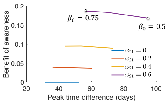
Figure S5: Benefit of adopted awareness versus the change in peak times as the infection rate changes. We let \beta_0 \in [0.5, 0.75] . The peak time difference is the difference between the time Locality 2 peaks and the time Locality 1 peaks. Let F_2(\omega_{21}, \Delta\beta) denote the final outbreak size at Locality 2 with respect to \omega_{21} and \Delta\beta . The benefit of awareness is defined as F_2(0, \Delta\beta) - F_2(\omega_{21}, \Delta\beta) where \Delta\beta \in [-0.125, 0.125] . Parameters of the dynamics (1)-(5): \mu = 1/3 , \delta = 1/4 , N_1 = N_2 = 1 , \alpha_1 = \alpha_2 = 1 , and \lambda_{12} = \lambda_{21} = 10^{-5} .
