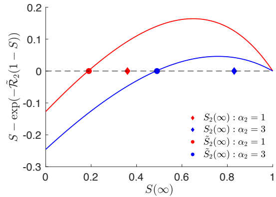
Figure S1: Lower bound values for S(\infty) . We assume low adopted awareness \omega_{21} = 1/2 . We let \mathcal{R}_1 = 2.5 and \lambda = 0.0001\% . (Top) Weak and (Bottom) strong response at the origin. Lines correspond to the left hand side of (10). Circle dots show the solution to (10), i.e., intersection of lines with zero. Diamond dots are S(\infty) values obtained by simulating the SEIR model in (1)-(4) with \beta_i in (5).
