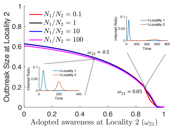
Figure S4: Outbreak size at locality 2 as a function of the population size ratio. Population size ratio is given by the ratio of initial population sizes between localities, i.e., N_1/N_2 . The epidemic and mobility dynamics are given by (1)-(4) and eq. (5) in the revised manuscript. Parameters: \beta_0 = 5/8 , \mu = 1/3 , \delta = 1/4 , \lambda_{12} = \lambda_{21} = 10^{-7} , and \alpha_1 = \alpha_2 = 1 .
