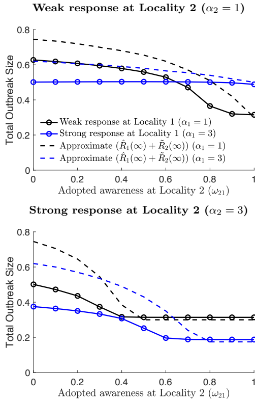
Figure 5: Total of outbreak sizes at localities 1 and 2 with respect to adopted awareness \omega_{21} . (Top) Weak ( \alpha_2 = 1 ) and (Bottom) strong ( \alpha_2 = 3 ) responses at Locality 2. Mobility is set to \lambda = 0.001\% . Weak and strong response at Locality 1 correspond to (\alpha_1 = 1) and (\alpha_1 = 3) , respectively. There exists a critical adopted awareness constant value in Top where the total outbreak size is lower in the scenario where both localities respond weakly compared to the scenario where Locality 1 has a strong response. The critical value for the adopted awareness constant value can be found by looking at the intersection of the solid black line with the solid blue line for the corresponding mobility value. When both localities respond strongly to the disease in Bottom figure, such a critical adopted awareness constant value does not exist.
