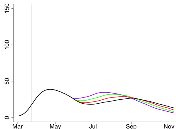
Figure 20: Expected deaths, x = 0.98 , R_2 = 1.3 , R_3 = 1.5
