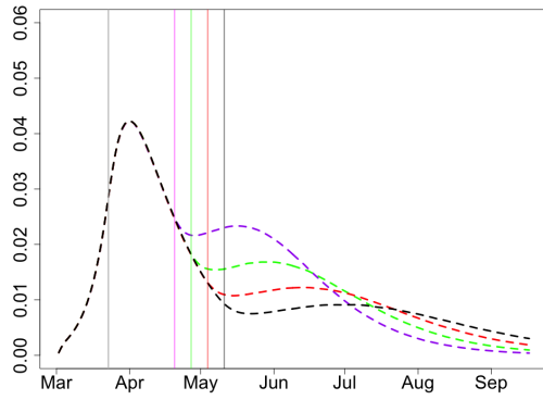
Figure 83: Proportion of infectious, x = 0.95 , R_2 = 1.75
