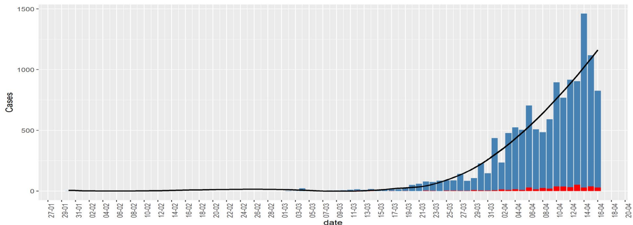
Figure 1: Bar chart of daily infected cases (blue) in India. Red bar denotes death. The black curve is a fitted smooth curve on the daily cases.
