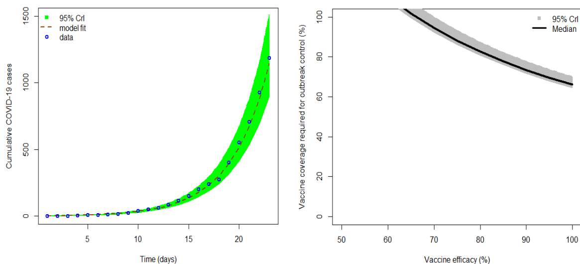
Figure 2: The first graph shows COVID-19 model fitting to cumulative cases where the green region is the 95% CrIs, the dashed brown line is the best model fit and the blue circles are the reported data for the cumulative number of COVID-19 cases in South Africa. The second graph shows the sensitivity analysis plot showing different vaccination coverages for different COVID-19 vaccine efficacy for South Africa. The dark grey regions are the 95% CrIs and the black line is the median.
