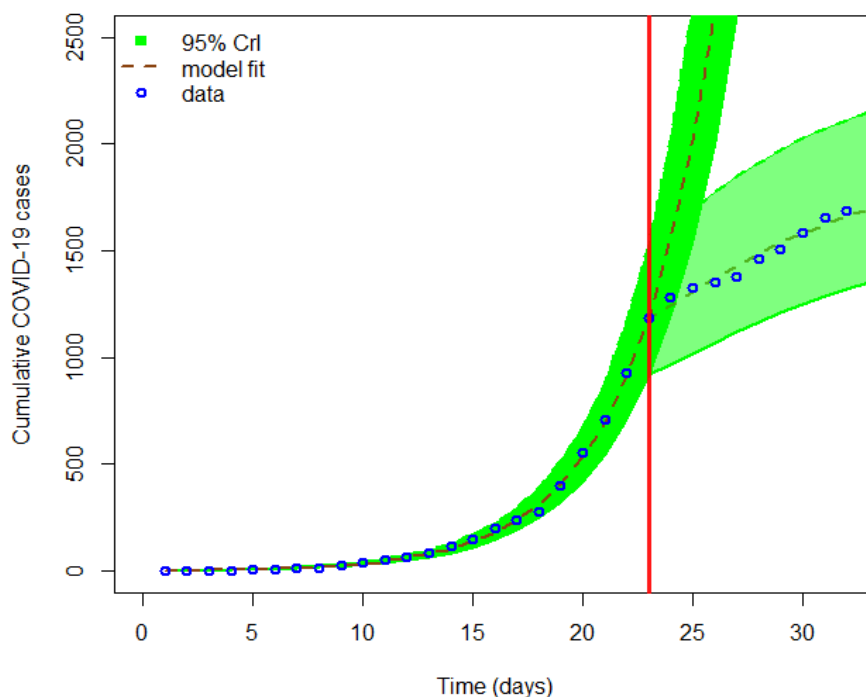
Figure 3: The first graph shows COVID-19 model fitting to cumulative cases where the green region is the 95% CrIs, the dashed brown line is the best model fit and the blue circles mark the reported data for the cumulative number of COVID-19 cases in South Africa. The red vertical line denotes the time when the lockdown was implemented by the government. The dark green region shows the trajectory the epidemic would have taken if a lockdown was not implemented and the light green region shows the trajectory of the epidemic after the implementation of a lockdown .
