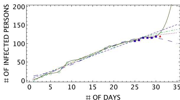
Figure 3: Data are the same as in Fig. 2. New data (red triangle) is not included in the fit. The continuous oliva curve is the fit from 1 to 25th days of [2, 3] data and 25th to 30th days of data from [2-4]. The dashed blue line is the linear fit in Eq. 3 while the dot-dashed green curve is the quadratic fit given in Eq. 4. The dotted red curve is the fit from the SI-like model used in [8, 9] while the large dashed green curve is the one from a gaussian-like fit used in [19].
