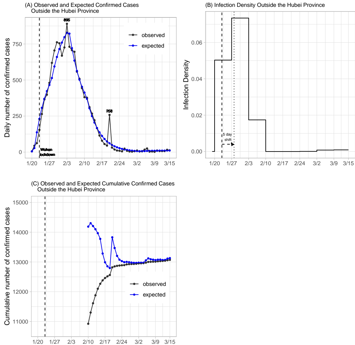
Figure 2: Plots of daily number of confirmed cases and infection density of confirmed cases in areas outside of the Hubei Province. Dashed and dotted lines indicate, respectively, the landmark time of Wuhan lockdown before and after accounting for a 5-day location shift.
