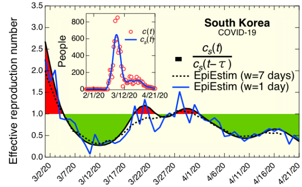
FIG. 2. The COVID-19 effective reproduction number for South Korea. The solid black line is from Eq. (2). The blue and dotted black lines are estimates from EPIESTIM using time windows of 1 day and 7 days, respectively. All calculations used \tau = 5.8 days, with a standard deviation (EPIESTIM case) of 2.9 days. The inset shows the reported incidence c(t) (red circles) and the smoothed curve c_s(t) .
