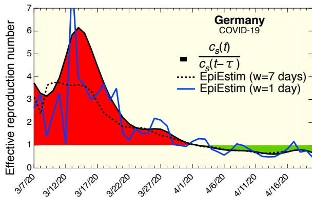
FIG. 5. The COVID-19 effective reproduction number for Germany. The solid black line is from Eq. (2). The blue and dotted black lines are estimates from EPIESTIM using time windows of 1 day and 7 days, respectively. All calculations used \tau = 5.8 days, with a standard deviation (EPIESTIM case) of 2.9 days.
