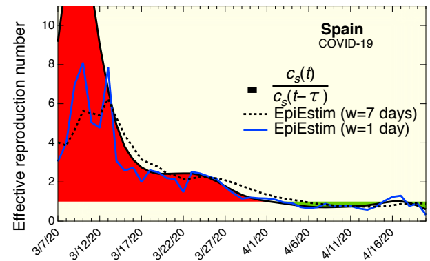
FIG. 3. The COVID-19 effective reproduction number for Spain. The solid black line is from Eq. (2). The blue and dotted black lines are estimates from EPIESTIM using time windows of 1 day and 7 days, respectively. All calculations used \tau = 5.8 days, with a standard deviation (EPIESTIM case) of 2.9 days.
