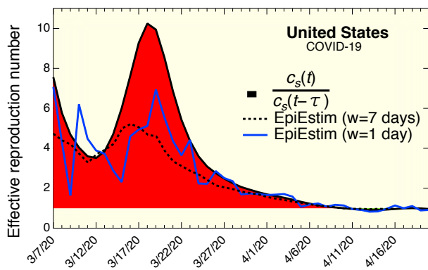
FIG. 6. The COVID-19 effective reproduction number for the United States. The solid black line is from Eq. (2). The blue and dotted black lines are estimates from EPIESTIM using time windows of 1 day and 7 days, respectively. All calculations used \tau = 5.8 days, with a standard deviation (EPIESTIM case) of 2.9 days.
