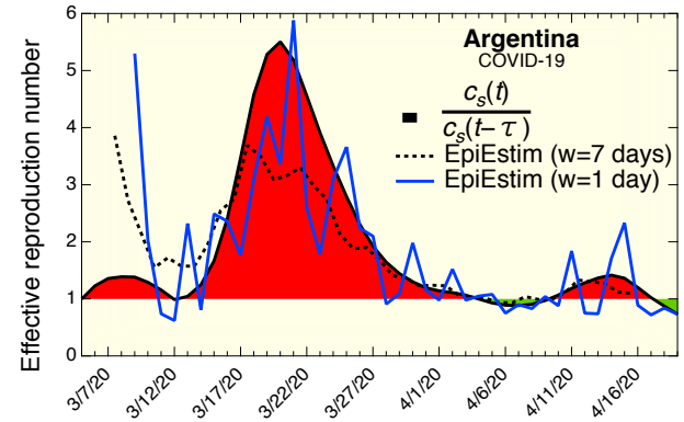
FIG. 7. The COVID-19 effective reproduction number for Argentina. The solid black line is from Eq. (2). The blue and dotted black lines are estimates from EPIESTIM using time windows of 1 day and 7 days, respectively. All calculations used \tau = 5.8 days, with a standard deviation (EPIESTIM case) of 2.9 days.
