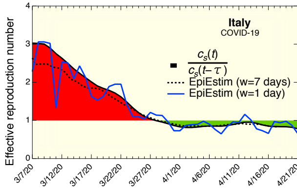
FIG. 4. The COVID-19 effective reproduction number for Italy. The solid black line is from Eq. (2). The blue and dotted black lines are estimates from EPIESTIM using time windows of 1 day and 7 days, respectively. All calculations used \tau = 5.8 days, with a standard deviation (EPIESTIM case) of 2.9 days.
