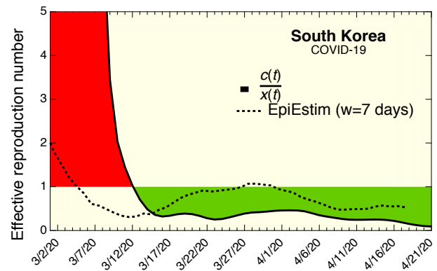
FIG. 1. Solid black line: effective COVID-19 reproduction number R_t for South Korea calculated from Eq. (1). Dotted line: R_t calculated with the package EPIESTIM using a mean infectious period \tau = 5.8 days with a standard deviation of 2.9 days and a time window of w = 7 days.
