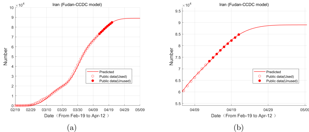
Figure 5: (a) Comparison of forecast results on April 12 and real data; (b) is an enlarged version of (a)
