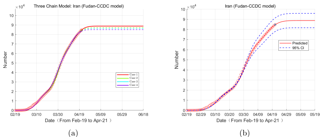
Figure 2: (a) Evolution of the increment of confirmed cases based on the three-chain Fudan-CCDC model. Red circles: data; Red lines: model predictions; (b) Evolution of the increment of confirmed cases based on the three-chain Fudan-CCDC model. Red circles: data; Red lines: model predictions; Blue dot line: 95% CI
