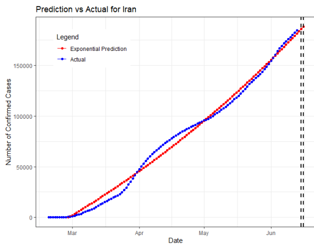
Fig. 3 Diagrammatic view of Predicted vs Actual number of confirmed cases in Iran. Left vertical dashed line represents 12 th June 2020 and right vertical dashed line represents 13 th June 2020.
