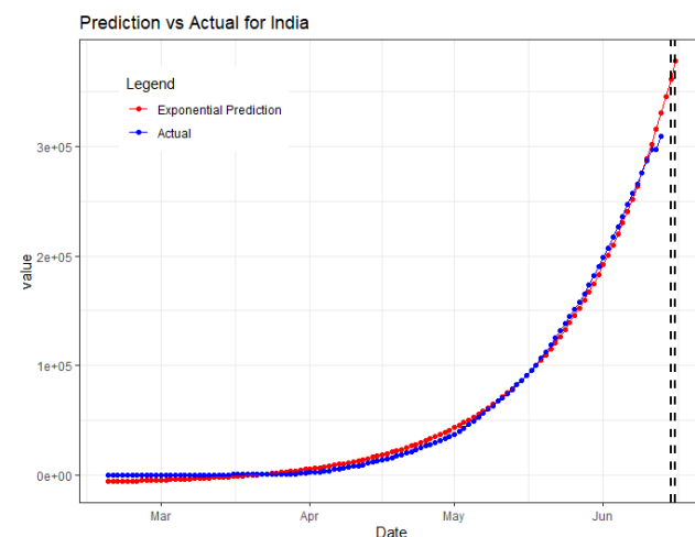
Fig. 2 Diagrammatic view of Predicted vs Actual number of confirmed cases in India. Left vertical dashed line represents 12 th June 2020 and right vertical dashed line represents 13 th June 2020.
