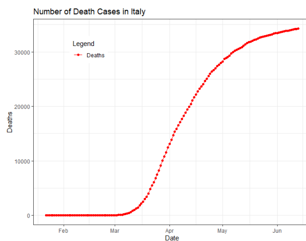
Fig. 6 Representation of the number of cases of Deaths recorded in Italy from 23 rd January 2020 to 11 th June 2020.
