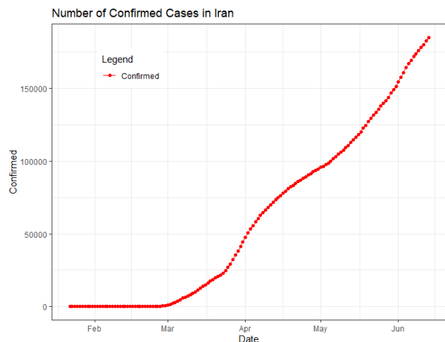
Fig. 7 Representation of the number of cases in Iran from 23 rd January 2020 to 11 th June 2020.
