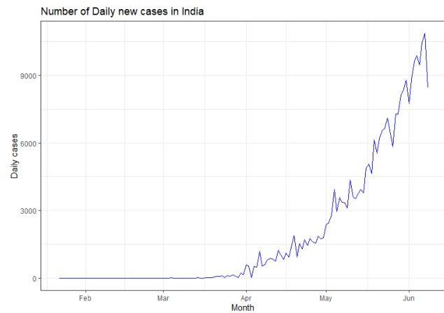
Fig. 8 Line plot of the number of new cases daily cases in India from the month of February to June.
