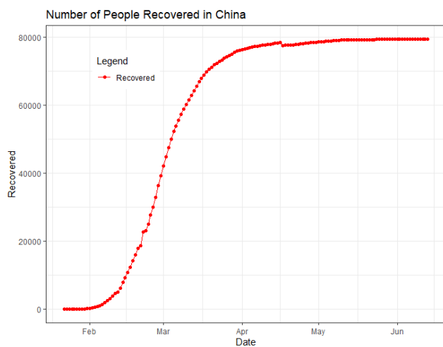
Fig. 5 Representation of the number of recovered cases recorded in China rate from 23 rd January 2020 to 13 th June 2020.
