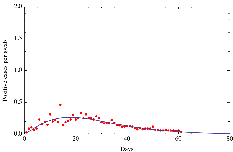
Fig. 1 Fit of the ratio of daily positive cases per swab obtained with a function of the type of the Planck's black body law with three parameters. The beginning date is February 25. Root Mean Square of the residuals is 0.0446
