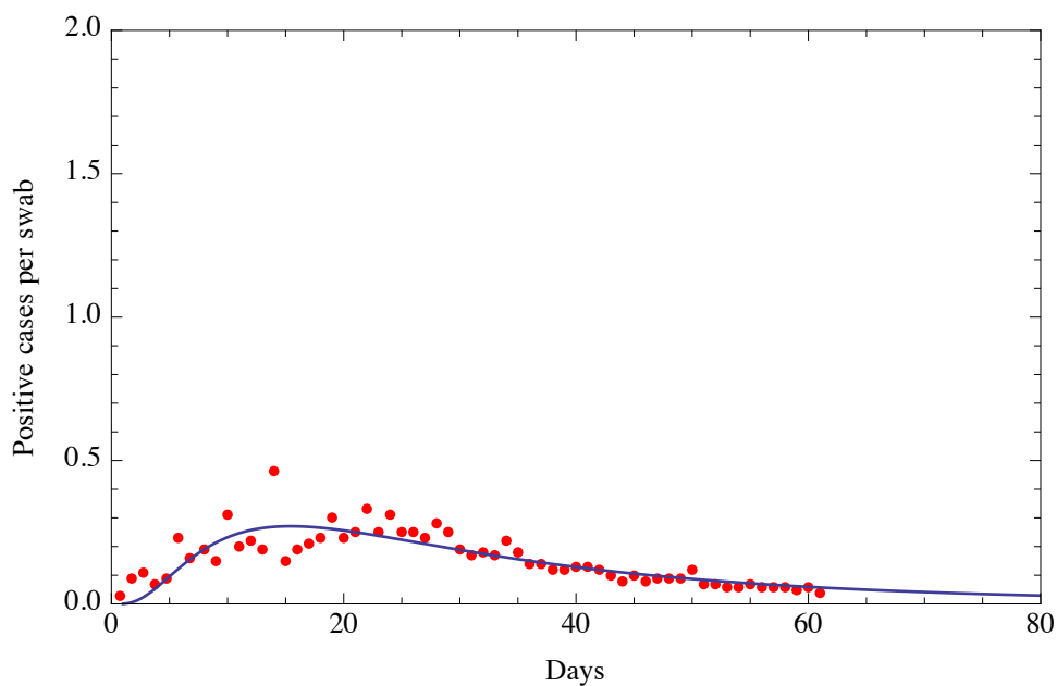
Fig. 2c Fit of the ratio of daily positive cases per swab obtained with a Beta distribution with two parameters. The beginning date is February 25. Root Mean Square of the residuals is 0.046
