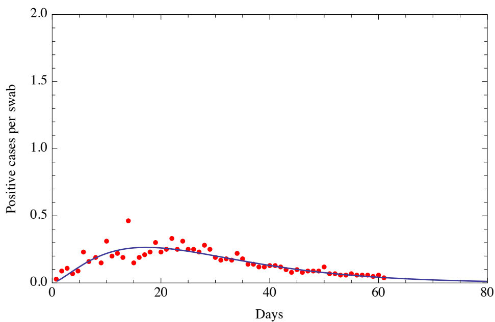
Fig. 2b Fit of the ratio of daily positive cases per swab obtained with a Gamma distribution with three parameters. The beginning date is February 25. Root Mean Square of the residuals is 0.0450
