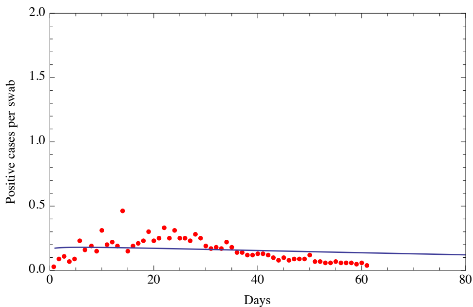
Fig. 2d Fit of the ratio of daily positive cases per swab obtained with a Weibull distribution with two parameters. The beginning date is February 25. Root Mean Square of the residuals is 0.082
