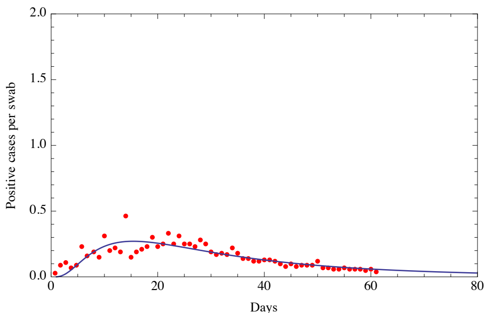
Fig. 2e Fit of the ratio of daily positive cases per unit swab obtained with a Lognormal distribution with three parameters. The beginning date is February 25. Root Mean Square of the residuals is 0.049
