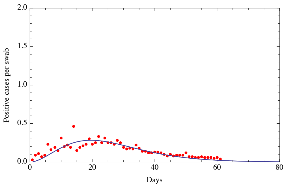
Fig. Fit of the ratio of daily positive cases per swab obtained with a function of the type of the Planck's black body law with two parameters, with the exponent of the time variable t equal to 3 as in the Planck's law. The beginning date is February 25. Root Mean Square of the residuals is 0.050
