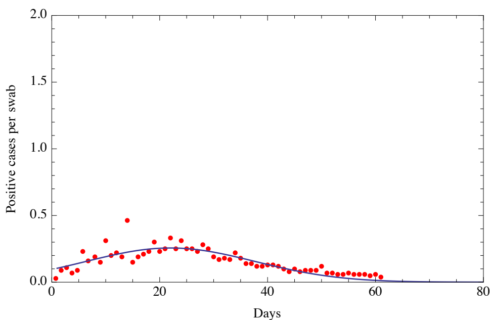
Fig. 2f Fit of the ratio of daily positive cases per swab obtained with function of the type of a Gauss function with three parameters. The beginning date is February 25. Root Mean Square of the residuals is 0.049
