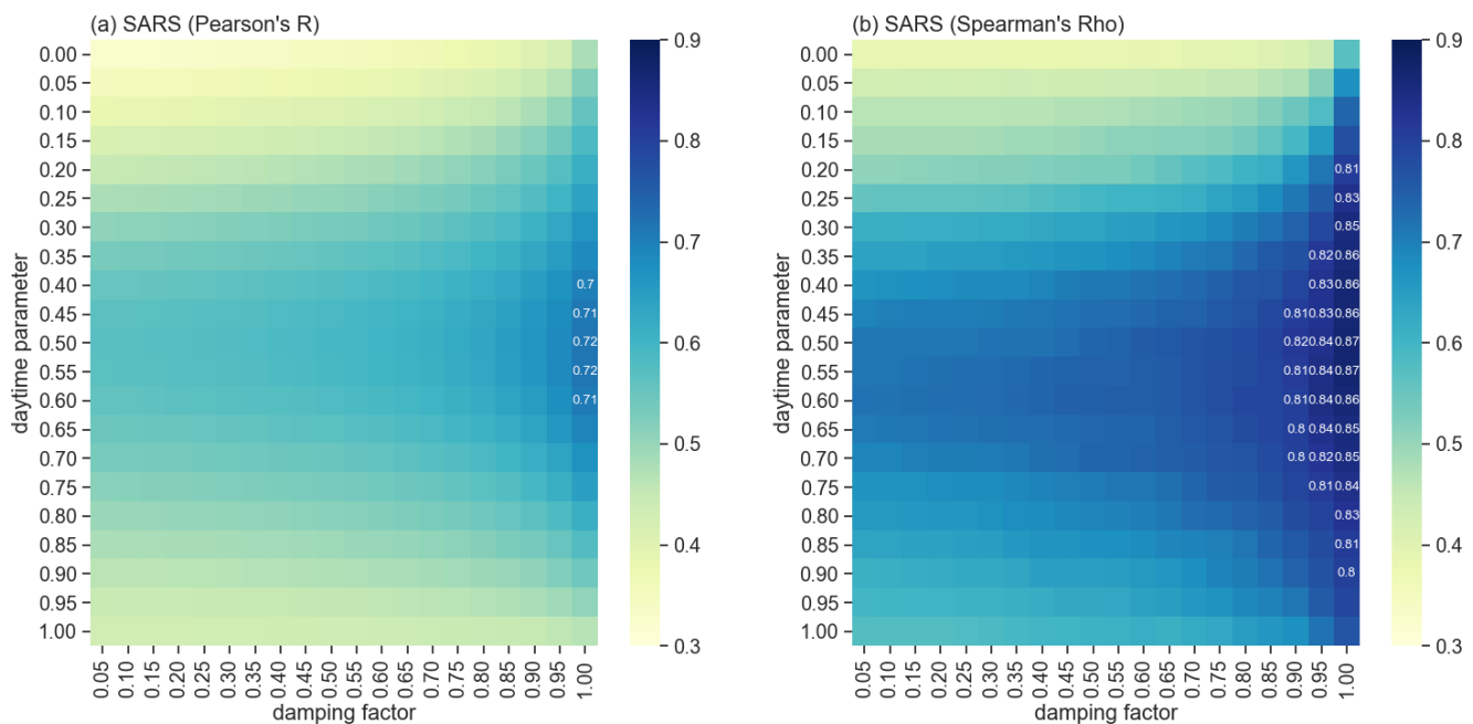
Figure 1. Sensitivity data for daytime (forward and backward movement) and damping factor values (effect of network topology compared to external factors). (a) Pearson's R, (b) Spearman's rho.
