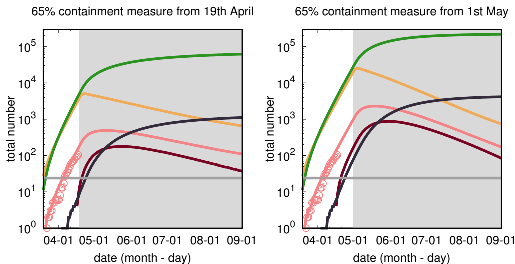
FIG. 3: Model results for containment measures reducing R_t by 65% with respect to R_0 . Left panel: measures enacted from the 19th of April, 2020. Right panel: measures enacted from the 1st of May, 2020. Different curves are different model predictions as in Fig. 2. The gray region marks the time interval where containment measures are imposed.
