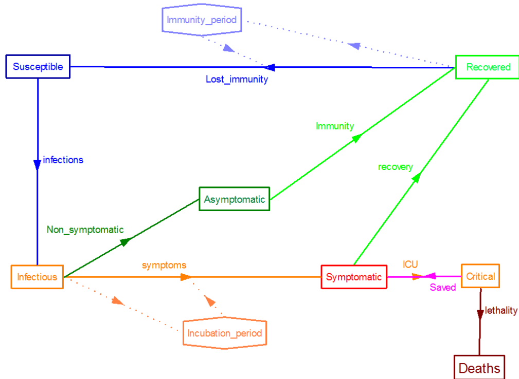
Figure 1: Example of a SIR type compartment model adapted to simulate the behaviour of SARS-CoV-2. In this case we assumed that immunity would be lost in a given period of time.
