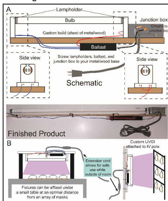
Figure 3: A) Schematic and finished product of the custom fixture that can be easily created to fit an existing UV-C bulb from a BSC. This custom fixture is one of the options depending on the end-user circumstances. The UV-C output should be measured using a UV-C meter for each individual configuration of sterilization set-up to determine the appropriate irradiation time. B) UVGI devices can be arrayed in a medical setting by affixing to available items such as tables or IV poles.
