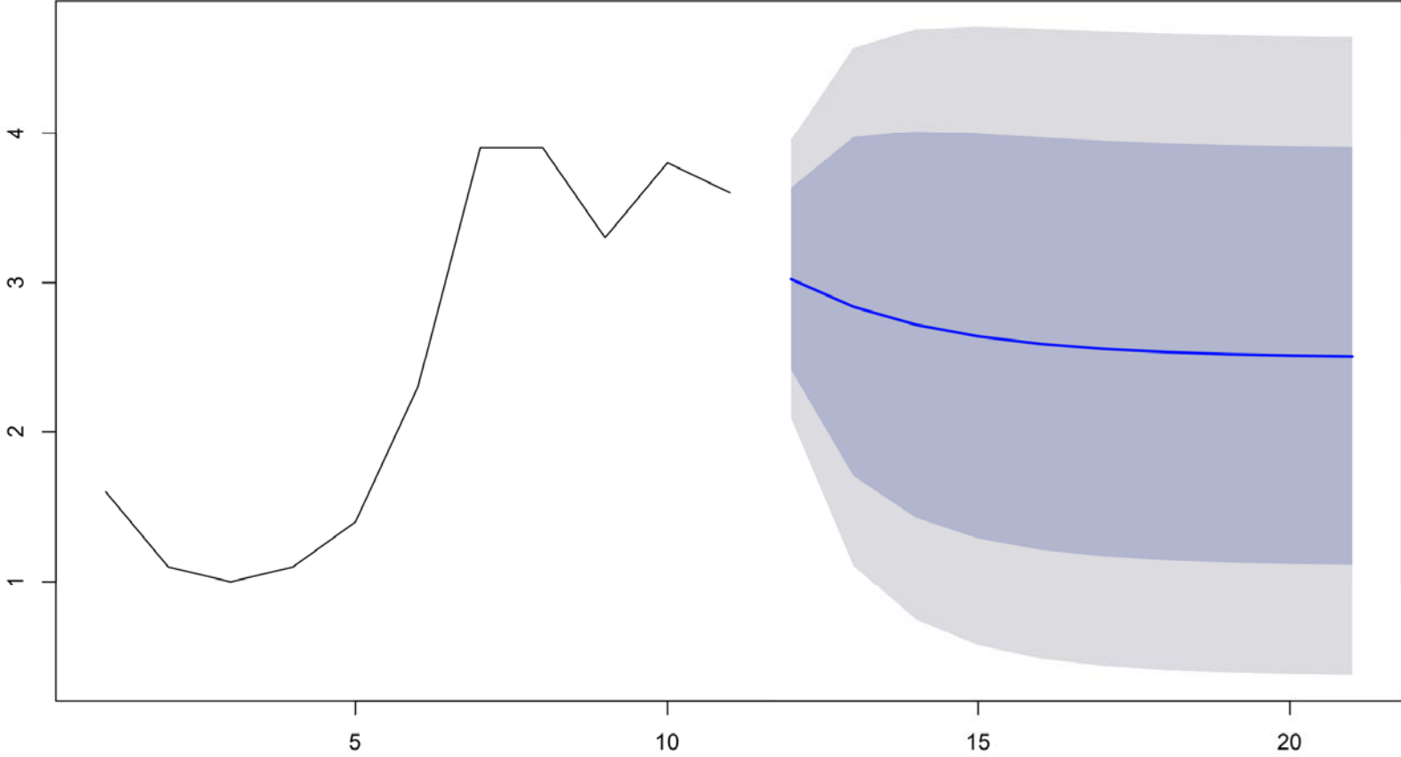
Forecasts from ARIMA(1,0,1) with non-zero mean
