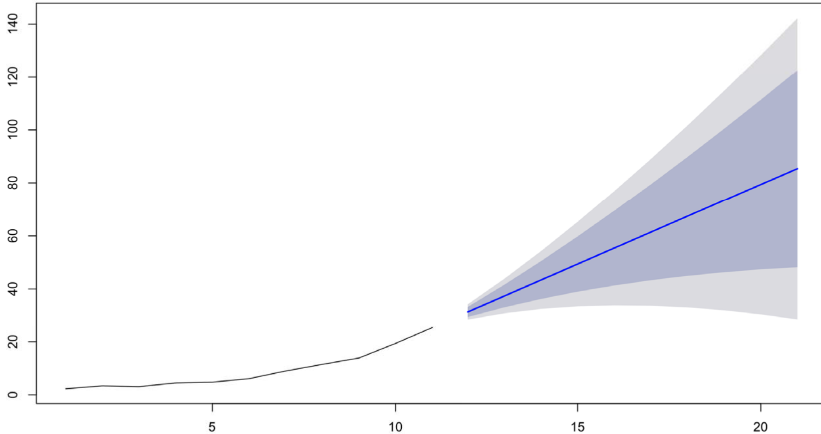
Forecasts from ARIMA(0,2,0)
