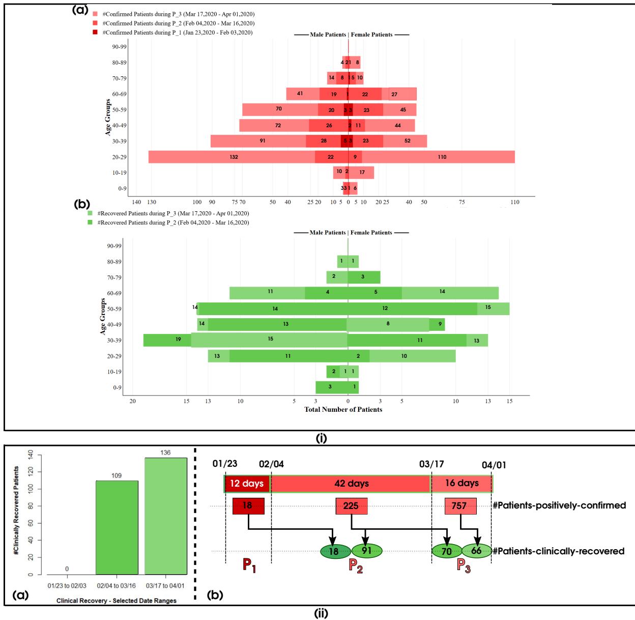
Figure 2: The entire period of our study is split into three periods: January 23-February 03 [ P_1 ], February 04-March 16 [ P_2 ], and March 17-April 01 [ P_3 ]. (i) Period-wise overlapped population pyramids to show the age-gender distribution of patients: ((i),(a)) 999 who were confirmed positive (excluding one 102-year old female patient who tested positive on April 01), and ((i),(b)) 245 who were clinically recovered. ((ii),(a)) shows the number of clinically recovered/discharged patients during the 3 periods. ((ii),(b)) shows the counts of patients grouped based on periods when they were confirmed positive and clinically recovered.
