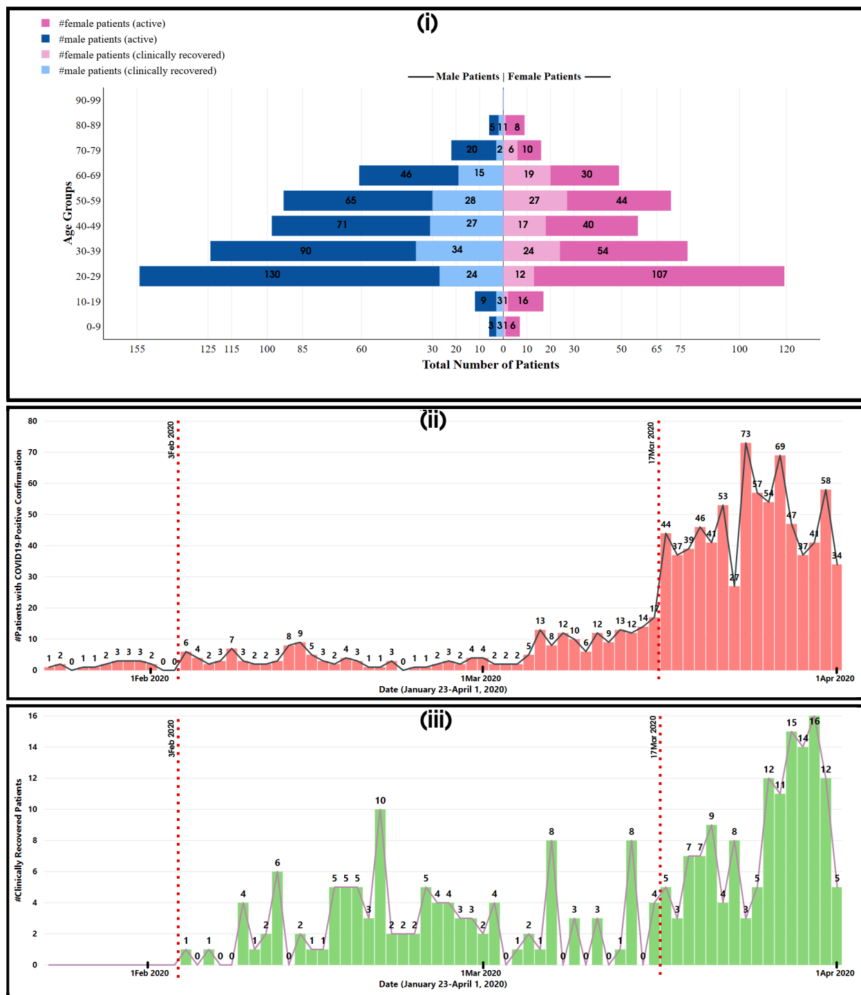
Figure 1: (i) Overlapped population pyramid of age-gender distribution of population of the 245 discharged and 754 active (i.e., COVID-19 positive but not discharged, including the deceased) during the same period (1 active patient who is a 102 years old female and confirmed positive on April 01, 2020, has been excluded in this population pyramid). Daily profile of count of patients in Singapore during January 23-April 01, 2020, (ii) who were confirmed positive for COVID-19, with a total of 1000, and (iii) who got clinically recovered and were discharged from the hospitals, with a total of 245. The red dotted lines indicate the three periods we have introduced in this work.
