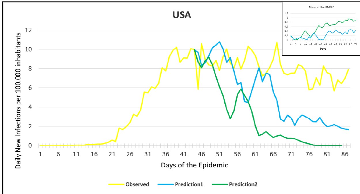
Figure 10. Observation and predictions for the United States of America (USA). The small graph in the upper right corner shows the daily error values calculated for the predictions.
