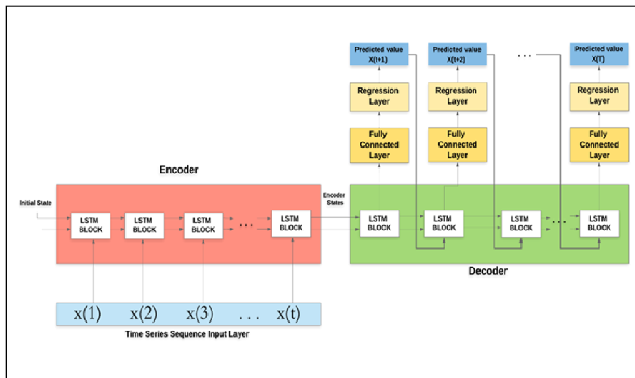
Figure 3. The Recurrent Neural Network (RNN) Architecture used for Prediction.
