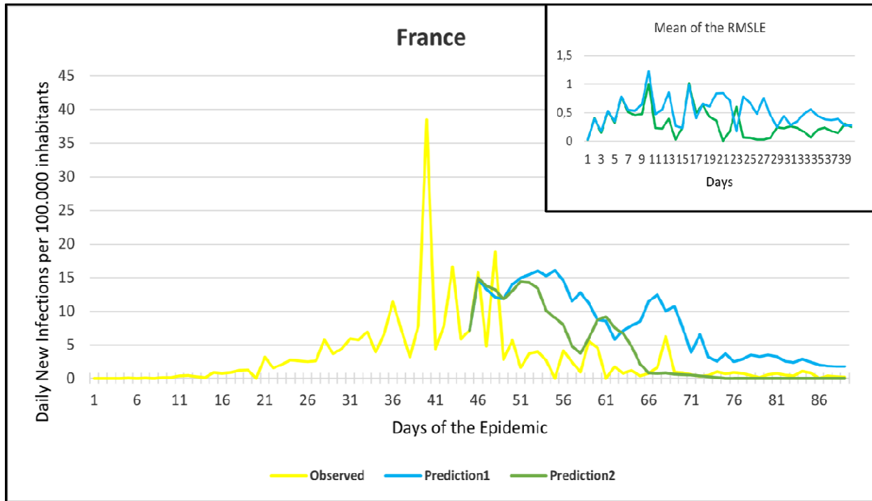
Figure 4. Observation and predictions for France. The small graph in the upper right corner shows the daily error values calculated for the predictions.
