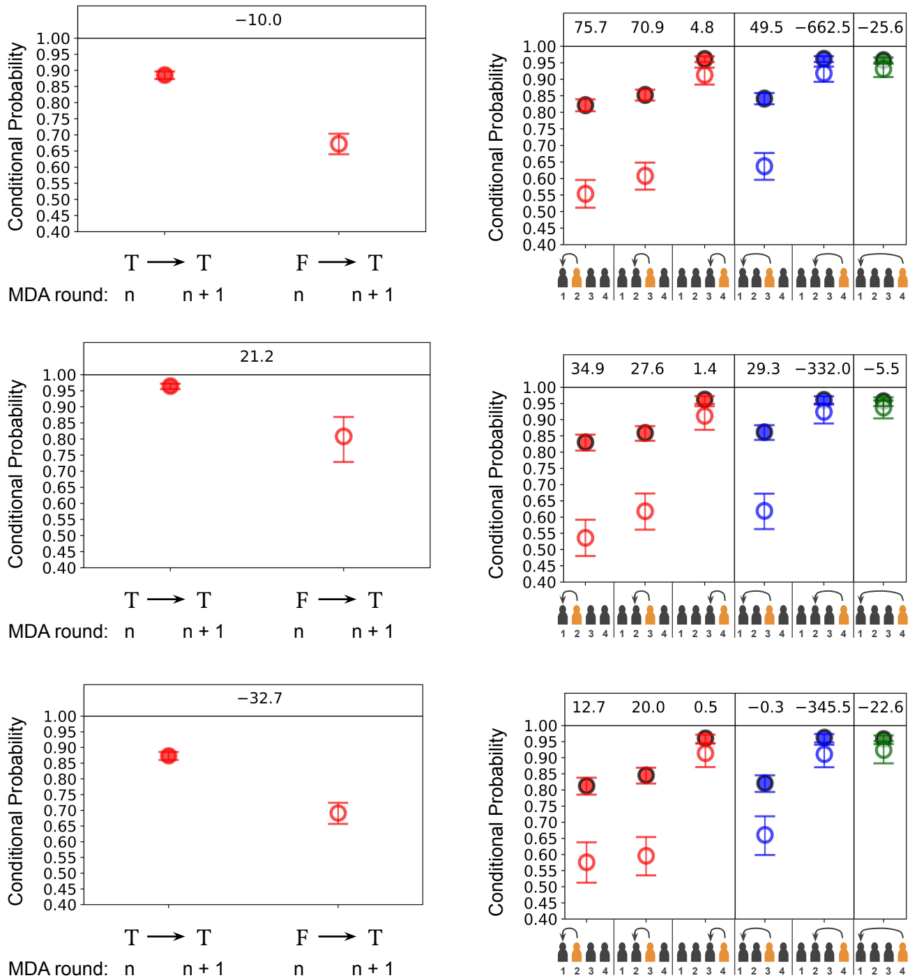
Fig 3. Left column: The maximum likelihood as well as the limits of the marginalised 95% credible region for the conditional probabilities of accepting treatment for any given pair of sequential rounds (these are hence homogeneous in time and the process is Markovian) given treatment (filled points) or non-treatment (hollow points) in a previous round. Right column: The same as the left column but with allowed time dependence in the conditional probabilities of accepting treatment in each respective round (highlighted in orange on the horizontal axes). In each case the components corresponding to a given round were measured assuming all other rounds were inferred to be from time-dependent past behaviour independent adherence and hence the likelihood is given in Appendix S1. Different colours for each point correspond to different lengths in time for the dependencies in behaviour. The datasets used are from the standard pre-SAC (0-4) age category from the TUMIKIA project where the: top row corresponds to the overall group; middle row corresponds to the male sub-group; and bottom row corresponds to the female sub-group.
