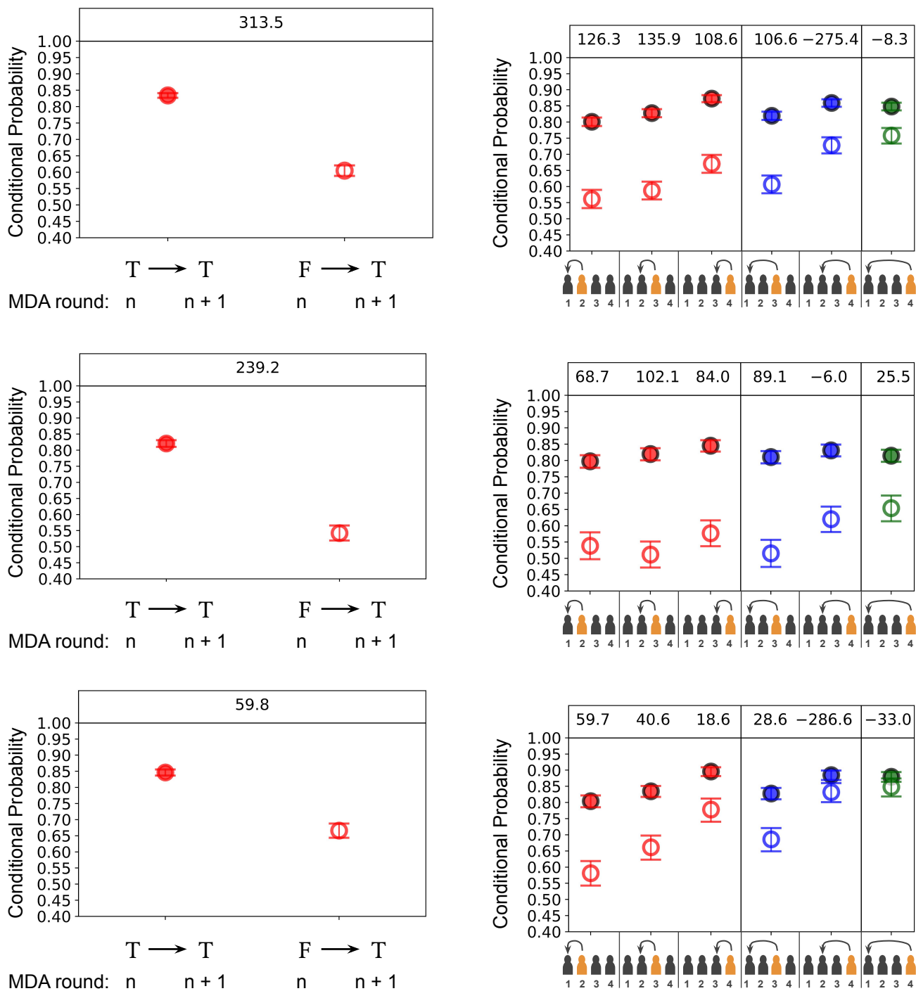
Fig 6. Left column: The maximum likelihood as well as the limits of the marginalised 95% credible region for the conditional probabilities of accepting treatment for any given pair of sequential rounds (these are hence homogeneous in time and the process is Markovian) given treatment (filled points) or non-treatment (hollow points) in a previous round. Right column: The same as the left column but with allowed time dependence in the conditional probabilities of accepting treatment in each respective round (highlighted in orange on the horizontal axes). In each case the components corresponding to a given round were measured assuming all other respective rounds were inferred to be from time-dependent past behaviour independent adherence and hence the likelihood is given in Appendix S1. Different colours for each point correspond to different lengths in time for the dependencies in behaviour. The datasets used are from the 30-49 age category from the TUMIKIA project where the: top row corresponds to the overall group; middle row corresponds to the male sub-group; and bottom row corresponds to the female sub-group.
