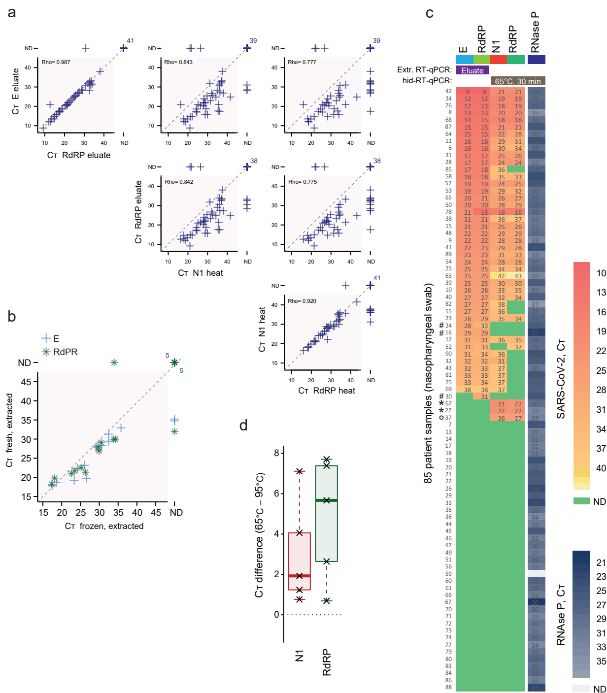
Figure 3. Diagnostic potential of SARS-CoV-2 hid-RT-qPCR. (a) Scatter plots of C_T values from clinical diagnostics performed on extracted RNA (y-axis) and hid-RTq-PCR (x-axis) of 85 nasopharyngeal swab samples, shown for different primer-probe set comparisons. Rho indicates Spearman correlation. ND: not detected. (b) Scatter plot of C_T values from 19 matched fresh (y-axis) and freeze-thawed (x-axis) extracted samples, using the E gene (cross) and RdRP (star) primer-probe sets. ND: not detected. (c) Heatmap of C_T from diagnostics performed on 85 clinical samples using extracted RNA (E, RdRP) and hid-RT-qPCR (N1, RdRP), ranked by E-gene C_T . Control for RNA degradation by RT-qPCR for RNase P transcripts in the same samples is show on the right. Two patients, marked with asterisk, negative in extraction-based routine diagnostics but positive by hid-RT-qPCR were later re-tested and confirmed to be SARS-CoV-2 positive (see Results). The patient marked with a ring was not re-tested. Three samples, marked with hash, were called COVID-19 positive by routine diagnostics, but not by any primer-set in hid-RT-qPCR. (d) Boxplots of C_T increase when the same nasopharyngeal swab samples were inactivated at 65°C for 30 min versus 95°C for 15 min.
