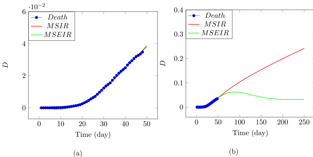
Figure 7: The fraction of the death calculated from coronavirus disease (Covid-19) data https://en.wikipedia.org/wiki/2020_coronavirus_pandemic_in_the_United_States . These data are collected from the official reports from state health officials between March 12 to April 28, 2020, and fitted with MSIR and MSEIR models for the removed. The population size 1.5 million was used for calculating the fractions. (a) small scale less than 50 days; (b) expanded to large scale. R^2 for both regressions are larger than 0.99.
