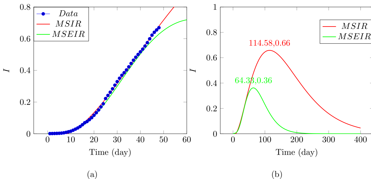
Figure 4: The fraction of the infected calculated from coronavirus disease (Covid-19) data https://en.wikipedia.org/wiki/2020_coronavirus_pandemic_in_the_United_States . These data are collected from the official reports from state health officials between March 12 to April 28, 2020, and fitted with MSIR and MSEIR models. The number of the infected individuals is divided by a population size 1.5 million to obtain the fraction. R^2 for both regressions are larger than 0.99.
