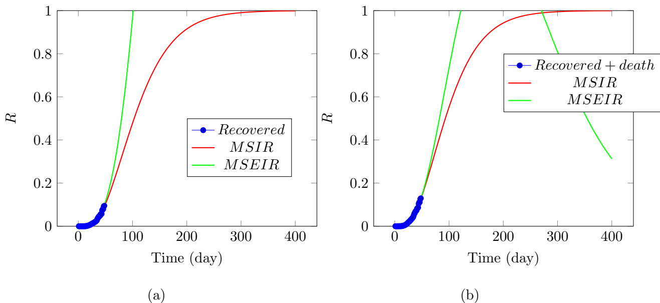
Figure 6: The fraction of the removed calculated from coronavirus disease (Covid-19) data https://en.wikipedia.org/wiki/2020_coronavirus_pandemic_in_the_United_States . These data are collected from the official reports from state health officials March 12 to April 28, 2020, and fitted with MSIR and MSEIR models for the recovered. The population size 1.5 million was used for calculating the fractions. (a) Only the recovered data are used for modeling; (b) Both the recovered and the death data are added together for modeling. R^2 for both regressions are larger than 0.99.
