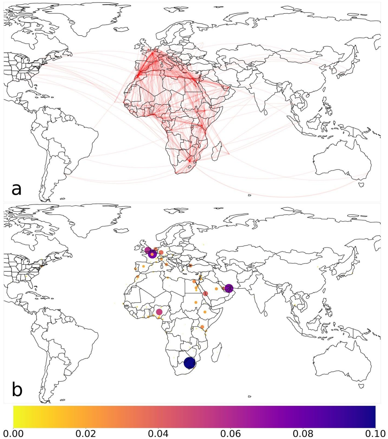
Figure 2: Airport connectivity and risk of outbreak initiation in Africa. a) A global map, overlaid with connections between global airports to an airport in Africa (red). Each connection represents the amount of air travel between locations to an airport in Africa, to which the curve opacity is proportional. b) The probability of passengers from different airports to initiate a COVID-19 outbreak in Africa, represented by color and circle area. Note that for visualization purposes, the color scale is truncated to [0,0.1].
