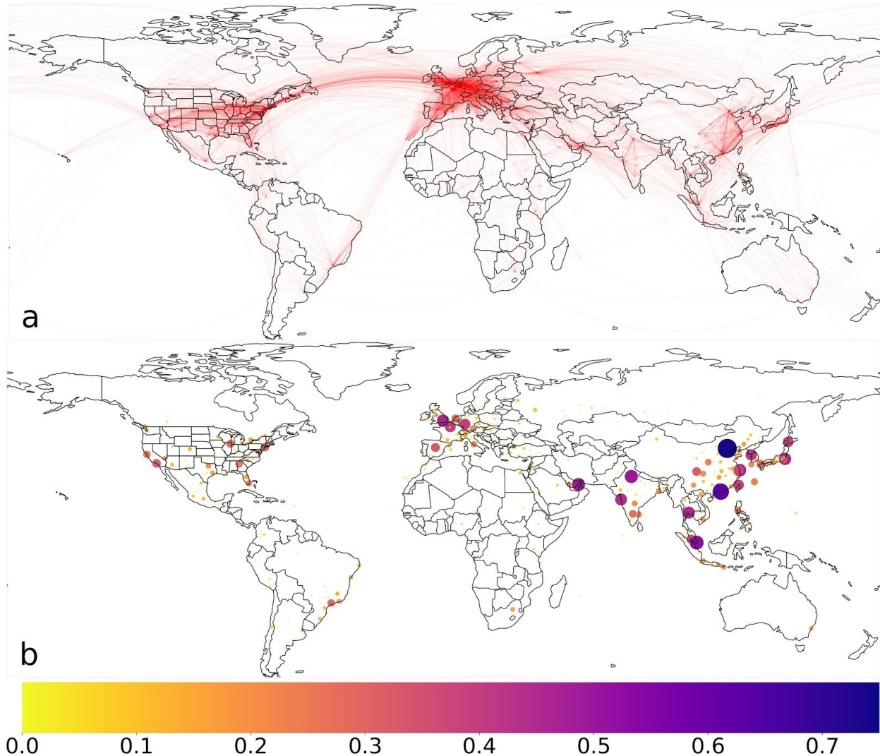
Figure 1: Global airport connectivity and risk of outbreak initiation. a) A global map, overlaid with connections between airports (red). Each connection represents the amount of air travel between locations, to which the curve opacity is proportional. b) The probability of passengers from different airports to initiate a COVID-19 outbreak somewhere around the world, represented by color and circle area. Note that for visualization purposes, the color scale is truncated to [0,0.75].
