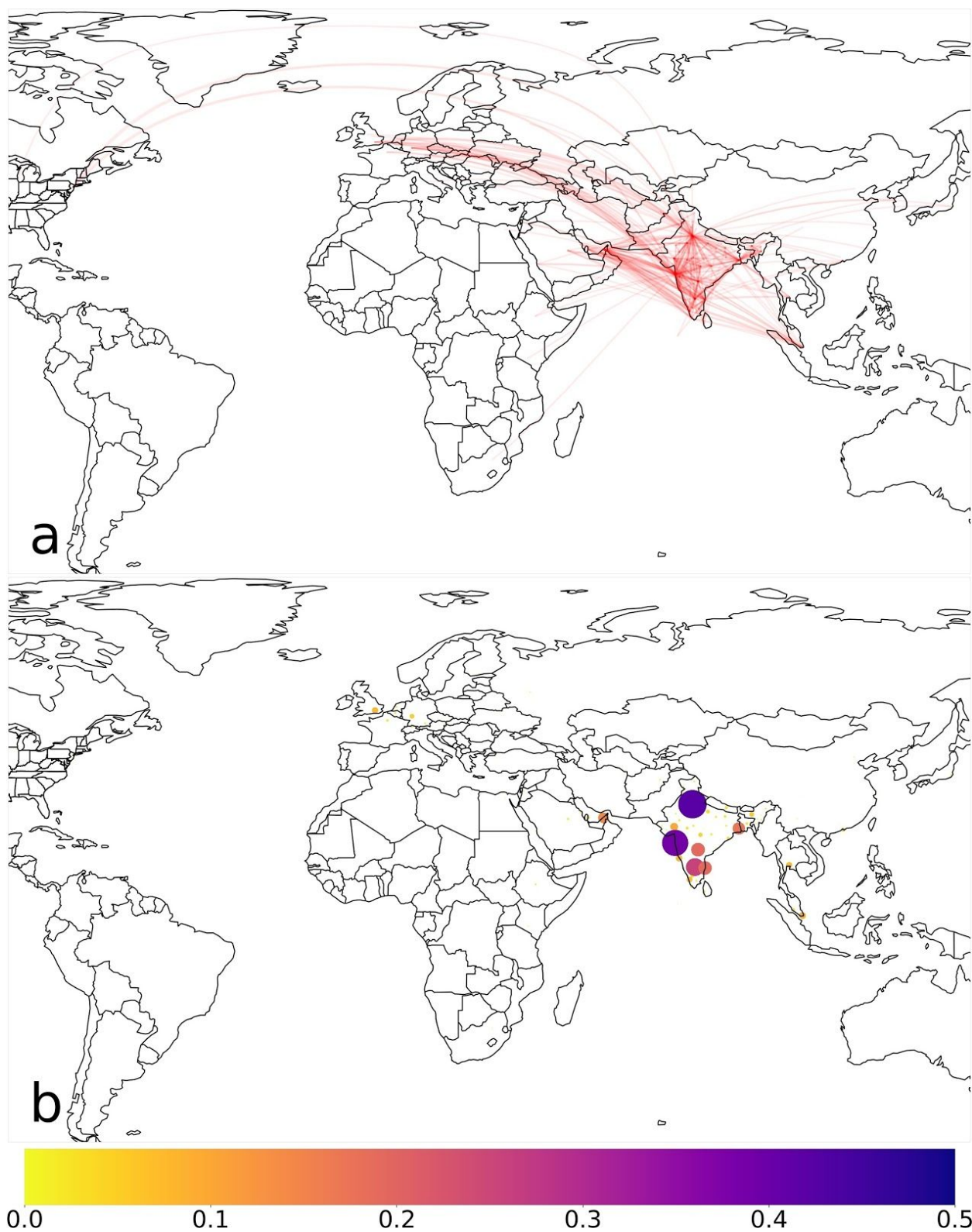
Figure 3: Airport connectivity and risk of outbreak initiation in India. a) A global map, overlaid with connections between airports worldwide to airports in India (red). Each
