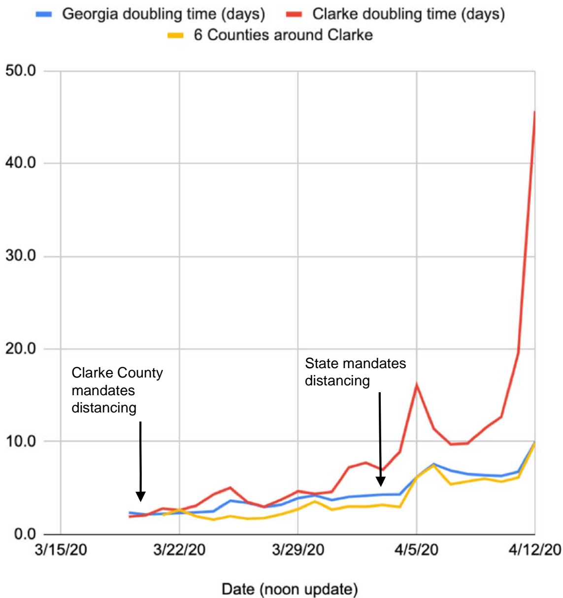
Figure 1. Doubling times for Clarke County, 6 surrounding counties, and the state of Georgia
