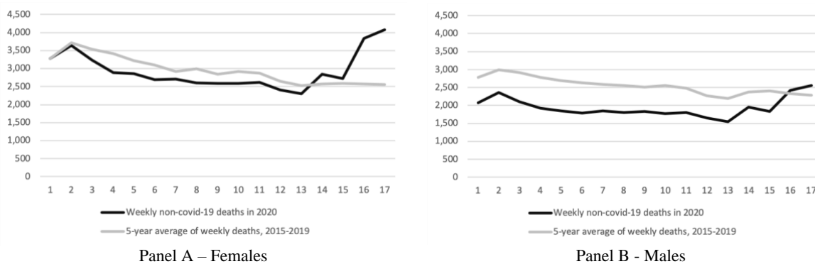
Figure A1.3 - Weekly deaths in England and Wales unrelated to covid-19, first 17 weeks, year 2020 and average of years 2015-2019, age group 85+
