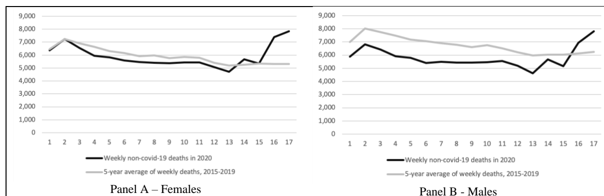
Figure 1 - Weekly deaths in England and Wales unrelated to covid-19, first 17 weeks, year 2020 and average of years 2015-2019. First covid-19 death in week 10. Based on ONS data published on 5 May 2020.
