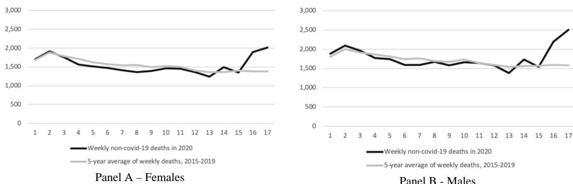
Figure A1.2 - Weekly deaths in England and Wales unrelated to covid-19, first 17 weeks, year 2020 and average of years 2015-2019, age group 75-84
