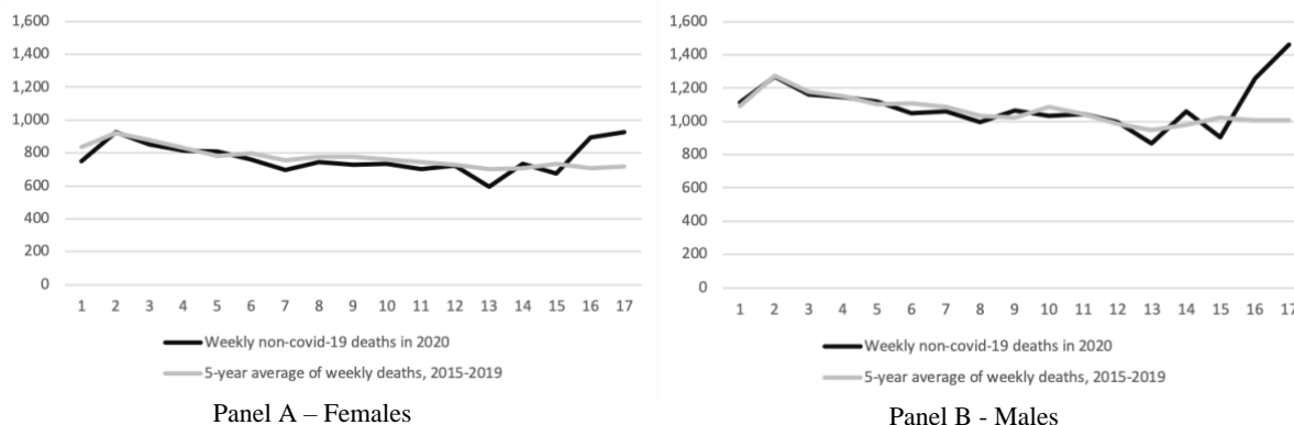
Figure A1.1 - Weekly deaths in England and Wales unrelated to covid-19, first 17 weeks, year 2020 and average of years 2015-2019, age group 65-74
