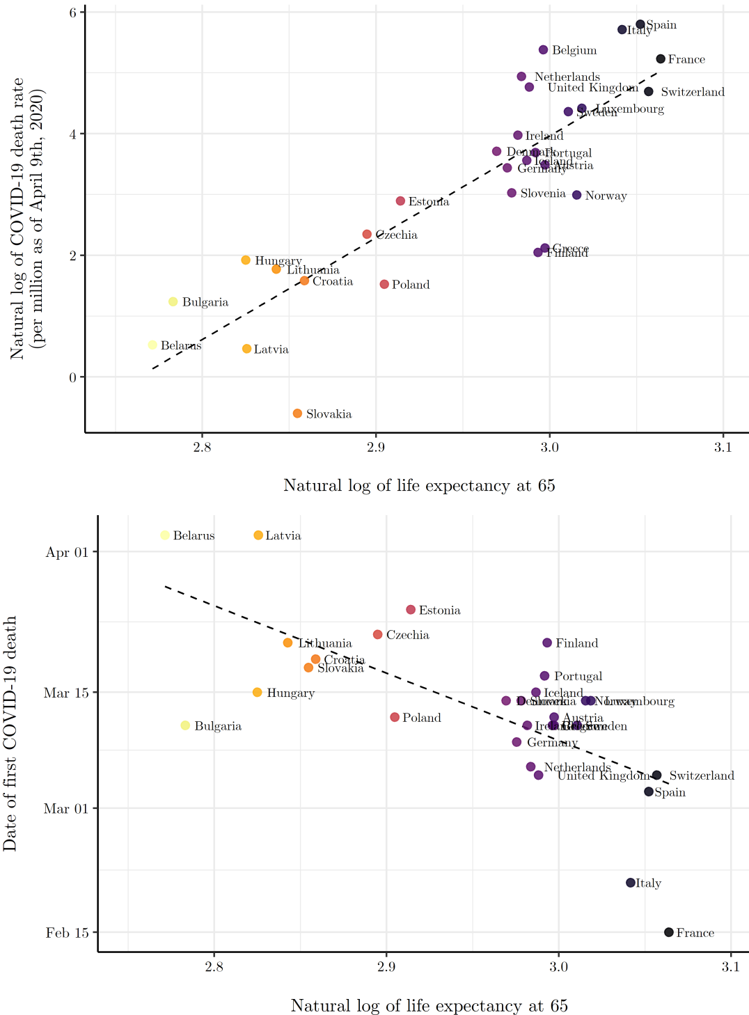
Figure 3: COVID-19 Death Rates (as of April 9th, 2020) and Epidemic Timing versus Life Expectancy at 65.
