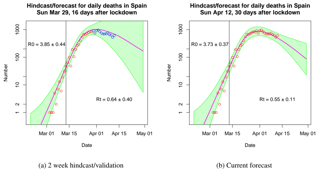
Figure 4. 2 week hindcast/validation and forecast for Spain Plot legend as for Figure 1
