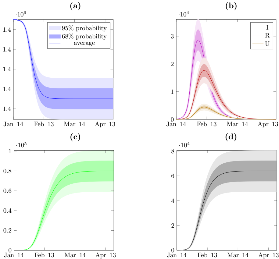
Figure 11: In figure (a) we plot the mean value and variance of S (susceptible) computed from the IBM. The dark blue area contains 68% of the trajectories, and the light blue area 95%. In figure (b) we plot the mean value and variance of I (infected), R (reported) and U (unreported) computed from the IBM. The dark areas contains 68% of the trajectories, and the light areas 95%. In figure (c) we plot the mean value and variance of RR (removed) computed from the IBM. The dark green area contains 68% of the trajectories, and the light green area 95%. In figure (d) we plot the mean value and variance of CR (cumulated reported) computed from the IBM. The dark gray area contains 68% of the trajectories, and the light gray area 95%. We use 500 independent runs of the IBM simulations. The parameters we used for both computations are the following: I_0 = 93 , U_0 = 5 , S_0 = 1.40005 \times 10^9 - (I_0 + U_0) , R_0 = RR_0 = CR_0 = 0 and f = 0.8 , \tau_0 = 3.3655 \times 10^{-10} , N = 26 , \mu = 0.148 , \nu = \frac{1}{7} , \eta = \frac{1}{7} , t_0 = 13.3617 .
