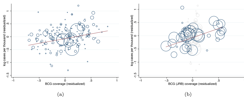
Figure 2. : Difference-in-Difference Analysis
