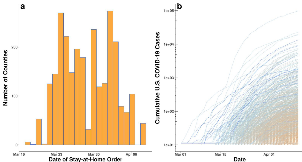
Figure 1. (a) Distribution of stay-at-home orders at the county level by date in the United States. (b) Log of cumulative confirmed COVID-19 active infections by county and date, gradient-colored by date of first case (blue = early to light blue = middle to orange = late).
