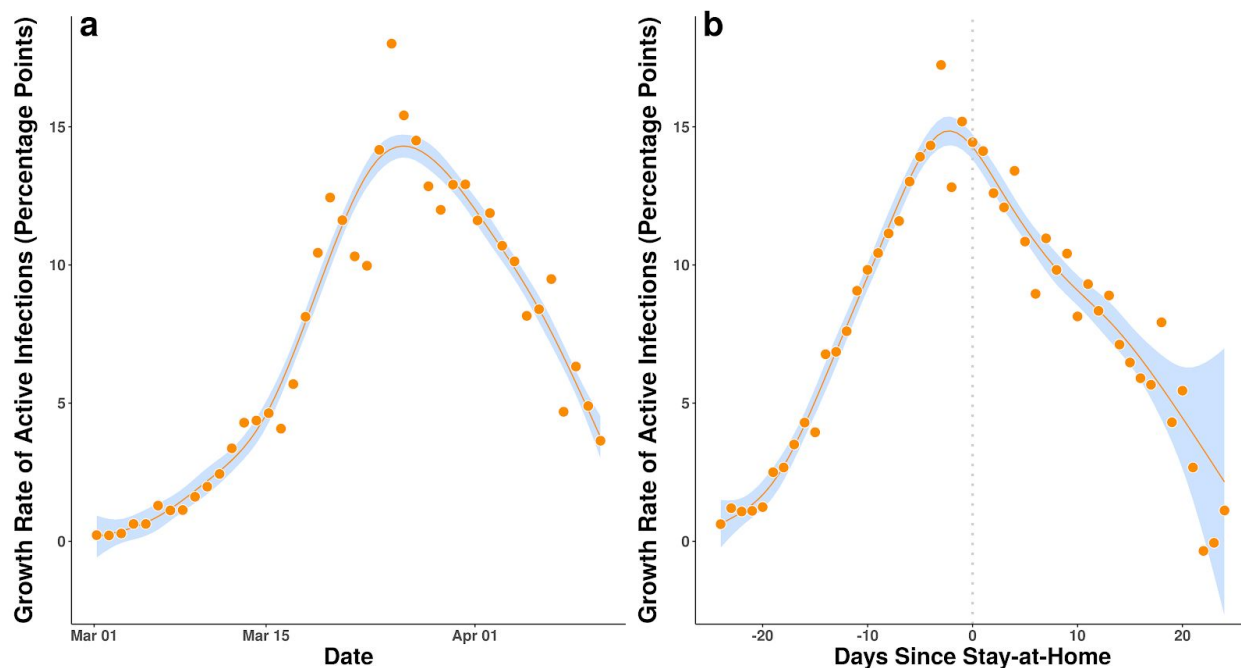
Figure 2. Mean U.S. daily growth in total active COVID-19 confirmed infections (a) by date, and (b) by the number of days before or after the stay-at-home order. Growth in active infections declines after stay-at-home orders towards 0, where the number of new active infections is approximately equal to the number of already-infected who recover. When growth goes below 0, the number of daily infections begins to decline.
