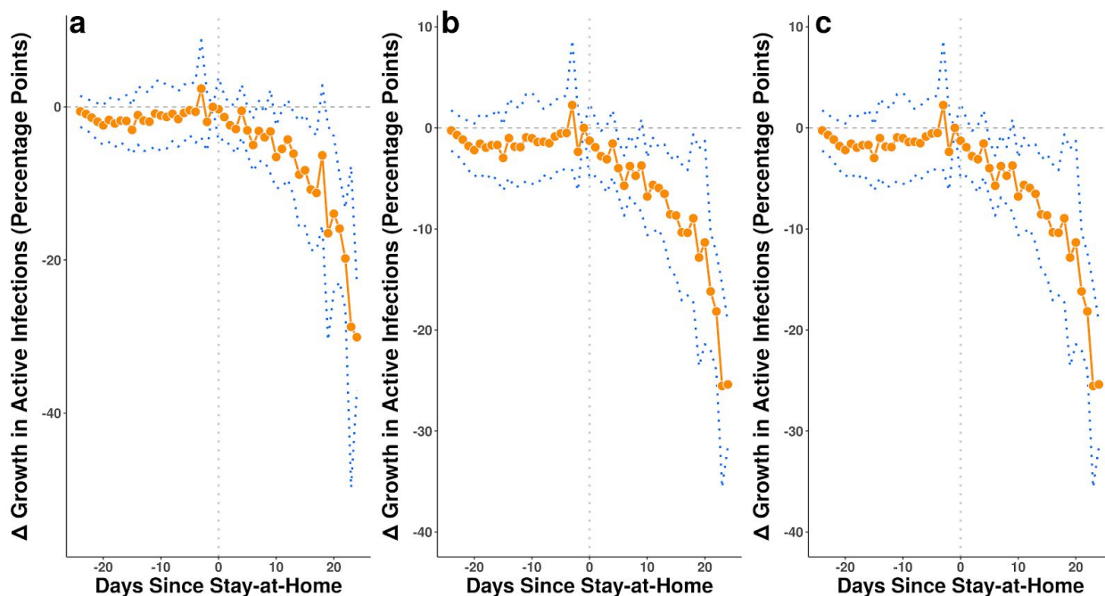
Figure 3. Estimated total effect of stay-at-home orders on the daily growth rate of COVID-19 confirmed infections in U.S. counties that implemented these orders, by the number of full days since the orders were issued. Estimates are derived from a fixed-effects regression of the daily growth rate of cases on days since initiation of the stay-at-home order as a categorical variable, where the reference category is the day prior to an order (Equation 3). Each panel of the figure displays a different model from Table 1, representing a different assumption about the number of days d cases remain active (a) d = 7 (Model 2); (b) d = 14 (Model 1); (c) d = 21 (Model 3). The models control for all county level and date fixed effects and for correlated observations with cluster-robust standard errors at the state level.
