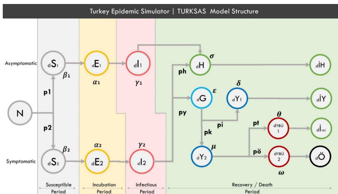
Figure 1: TURKSAS model structure. In a time section; N : Total population; d : delta (expressing the change of the related cluster over time) S - E - I : The number of Susceptible-Exposed-Infected people, respectively, in the relevant time section. H : Infected who have mild symptoms. I_H : Those who have recovered with mild symptoms. G : Infected and have not yet applied to the hospital. Y : Infected who apply to the hospital and occupied non-ICU beds. I_Y : Those who have recovered from the hospital as discharged. I_{YBU} : Those who have recovered from ICU. YBÜ1 : Those who will recover in ICU. YBÜ2 : Those who will die in ICU. Ö : Those who died. For other parameters, see. Mathematical Equation of the Model
