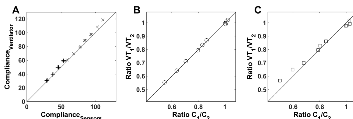
Figure 2. Comparisons of compliance and tidal volumes. A: compliances determined via the ventilator against compliances determined via external sensors. +: one compartment disconnected via pinching off the tracheal tube, x: both compartments connected. B: ratios of tidal volumes in compartments (VT1 and VT2) against ratios of compliances of the compartments (C1 and C2) as determined from external sensors. C: ratios of tidal volumes in compartments (VT1 and VT2) against ratios of compliances of the compartments (C1 and C2) as determined from the ventilator.
