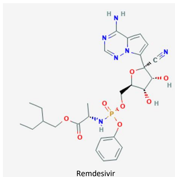
Figure 5 Potential drug candidate to treat COVID-19 manufactured by Gilead Sciences to treat COVID-19, remdesivir (PubChem Identifier: CID 121304016, URL: https://pubchem.ncbi.nlm.nih.gov/compound/121304016#section=2D-Structure )
