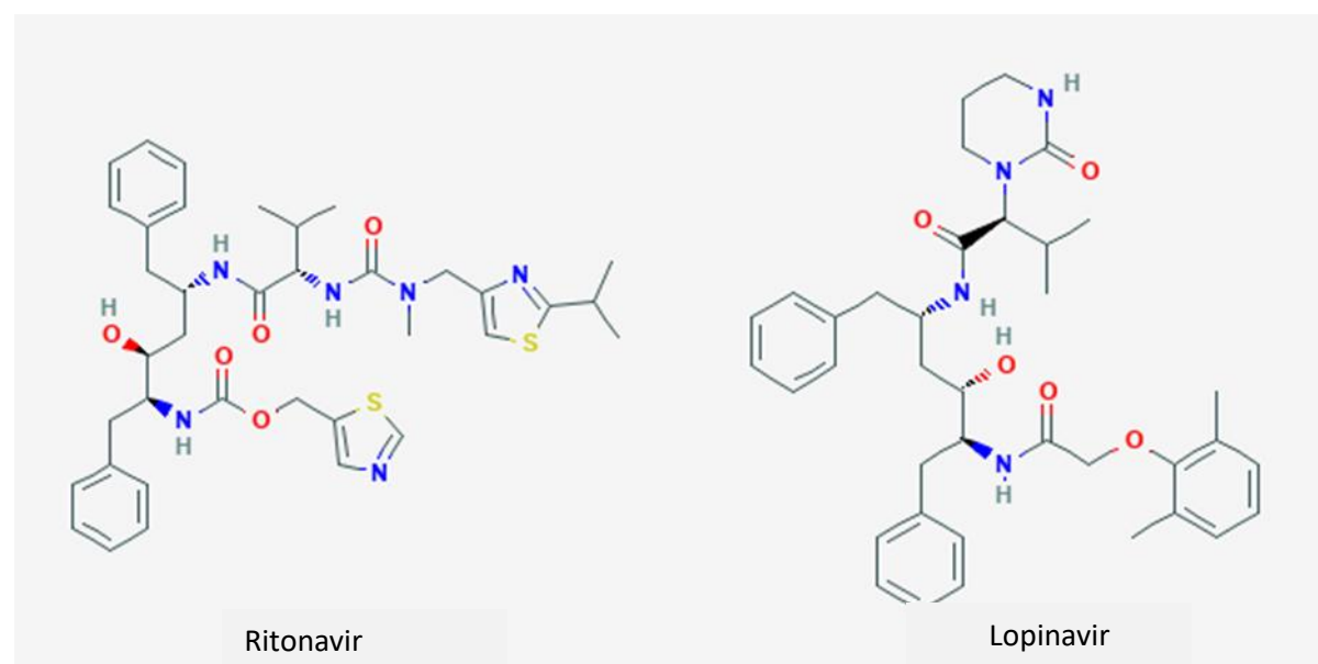
Figure 3 Chemical structure of HIV protease inhibitor, ritonavir (PubChem Identifier: CID 392622, URL: https://pubchem.ncbi.nlm.nih.gov/compound/392622#section=2D-Structure )
