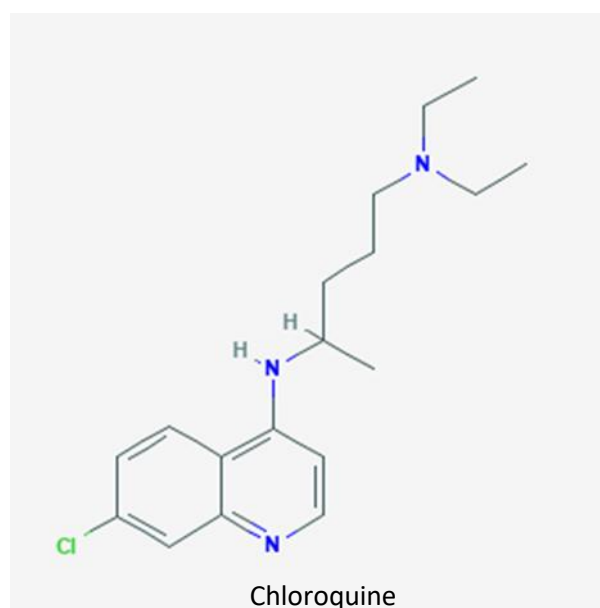
Figure 7 Chemical structure of chloroquine, which was initially used as an anti-malarial agent (PubChem Identifier: CID 2719, URL: https://pubchem.ncbi.nlm.nih.gov/compound/2719#section=2D-Structure )
