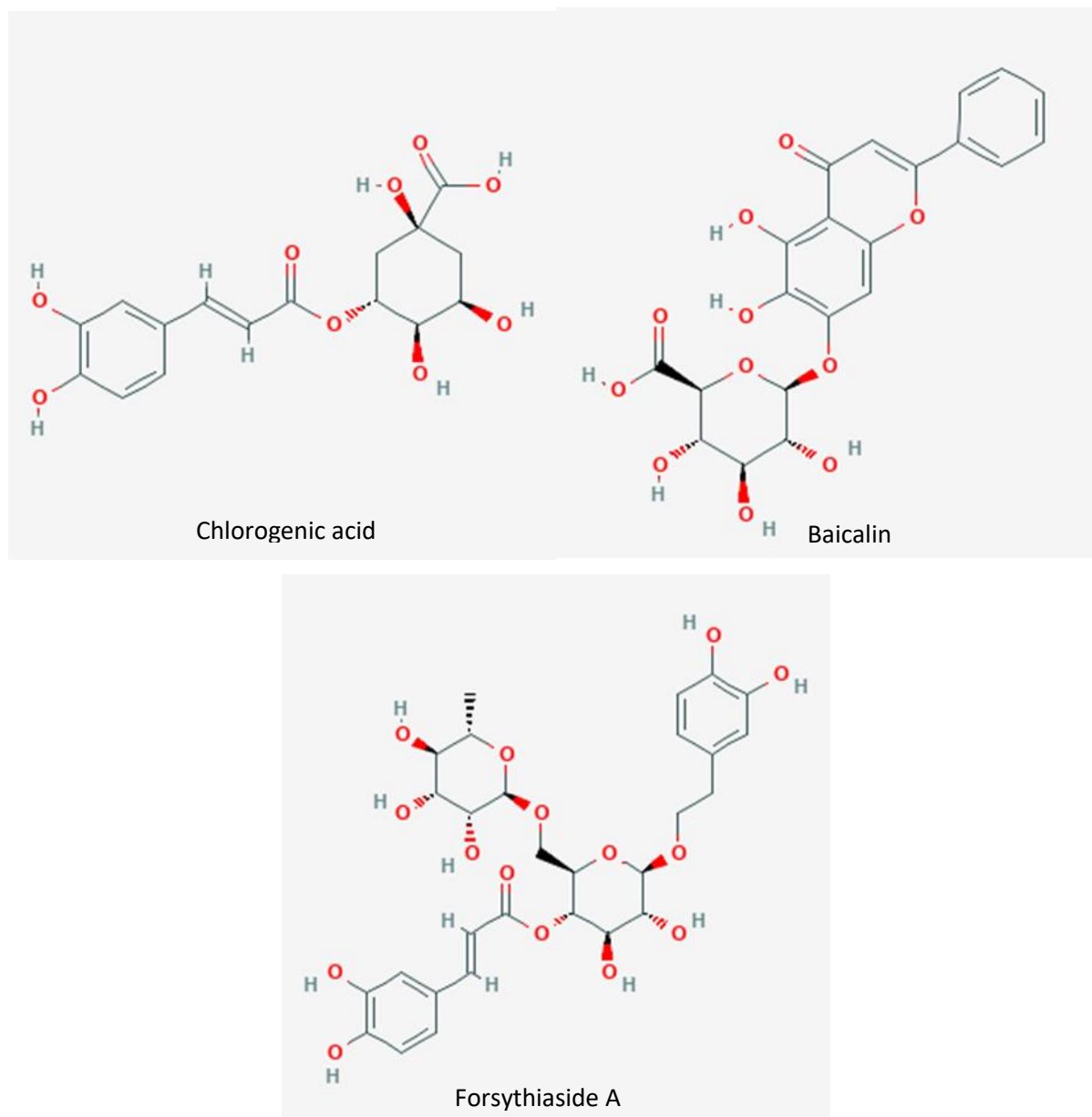
Figure 8 Chemical constituents of Shuang Huang Lian Kou Fu Ye , which responsible for the antiviral mechanism of action: Chlorogenic acid (PubChem Identifier: CID 1794427 URL: https://pubchem.ncbi.nlm.nih.gov/compound/1794427#section=2D-Structure ), baicalin (PubChem Identifier: CID 64982 URL: https://pubchem.ncbi.nlm.nih.gov/compound/64982#section=2D-Structure ), and
