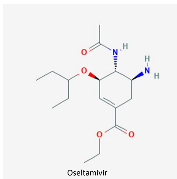
Figure 4 Oseltamivir, Synthetic prodrug for treatment of the Influenza virus (PubChem Identifier: CID 65028, URL: https://pubchem.ncbi.nlm.nih.gov/compound/65028#section=2D-Structure )
