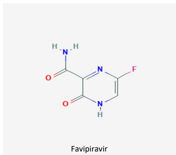
Figure 6 Favipiravir, nucleotide analogue manufactured by Toyama Chemicals for inhibiting a wide range of RNA viruses proliferation (PubChem Identifier: CID 492405, URL: https://pubchem.ncbi.nlm.nih.gov/compound/492405#section=2D-Structure )
