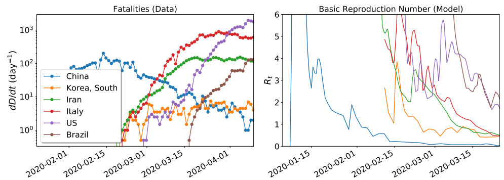
Fig 3. Left: The time series of fatalities for a number of countries. Right: the time derivative of the curve of fatalities is converted into \mathcal{R}(t) according to Eq. (19).
