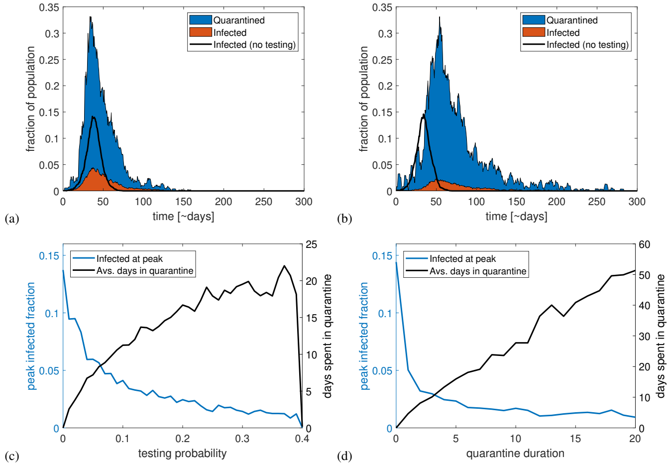
Figure 3. (a) and (b) show examples of epidemic trajectories for a quarantine length of 5 days and a daily testing probability of 10 and 20 % respectively. The blue section of the curve shows the fraction of people who are in quarantine, while the orange section shows the fraction who are ill. (c) and (d) show the peak fraction of population infected (left y-axis) and average time spent in quarantine (right y-axis) as a function of testing chance and quarantine length. The number of days in quarantine was calculated using our standard group sizes which connect each person to approximately 20 others. The average quarantine time scales proportionally with this assumed connectivity. (c) With a quarantine length of 5 days, it is possible to reduce the peak number of infected by ten percentage points, corresponding to a 70 % drop, if the probability of infected people being tested is only 10 % per day of illness. However, the price of this is that each person is on average quarantined twice during the epidemic. If testing is more widespread, the epidemic peak can be reduced, until it finally becomes unstable at a testing probability of around 40 % per day. If it is possible to completely eliminate the epidemic, the number of days spent in quarantine is similarly reduced. (d) Epidemic peak and time spent in quarantine as a function of quarantine length for a testing probability of 20 % per day. The average time spent in quarantine increases linearly with the length of quarantine. On the contrary, the effect of quarantine on the peak height appears to stagnate at approximately five days.
