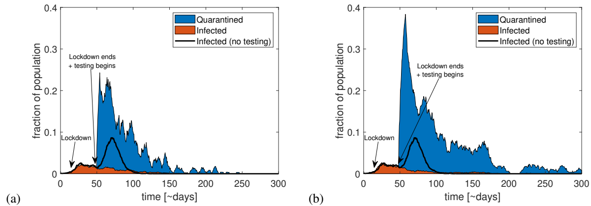
Figure 4. Various trajectories of the epidemic. (a) shows a possible course of an epidemic where restrictions in public and work life (by 75 %) are implemented when 1 % are infected and lifted after 30 days, being replaced by a testing and tracing regime with a testing probability of 20 % per day and quarantine duration of 5 days. The black line shows the fraction of infected if no testing is implemented. We see that this level of testing and quarantine is sufficient to prevent a resurgence of the epidemic. (b) is similar, but here quarantine lasts 10 days. This is about as effective as (a), but costs a lot more in terms of number of people in quarantine.
