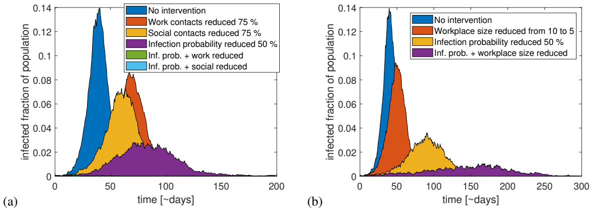
Figure 2. (a) Comparison of various strategies with and without a reduction in transmission probability per encounter. It can be seen that work and social contacts play roughly the same part in disease transmission. A reduction of infection probability makes the strategies relatively more effective. Reducing work contacts, for example, reduces the peak height by roughly 40 % (relative to no intervention) if infection probability is high. If the infection probability is lowered, the strategy completely eliminates the epidemic. (b) A similar comparison of the effects of reducing workplace sizes by half. This strategy is also relatively more effective if infection probability is reduced. The strategy reduces peak height by 75 % at a lowered infection probability versus only 35 % if infection probability remains high.
