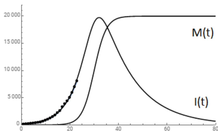
Fig. 7. Comparison of the dynamics of the number of cases during the COVID-19 epidemic in Russia according to the SIMR model (the solid line I(t) ) with statistical data [3] (the line with dots). The SIMR parameters are taken as m=0.39 , \beta=0.40 , \gamma=0.075 . Saturation of M(t) corresponds to 100% hidden immunization.
