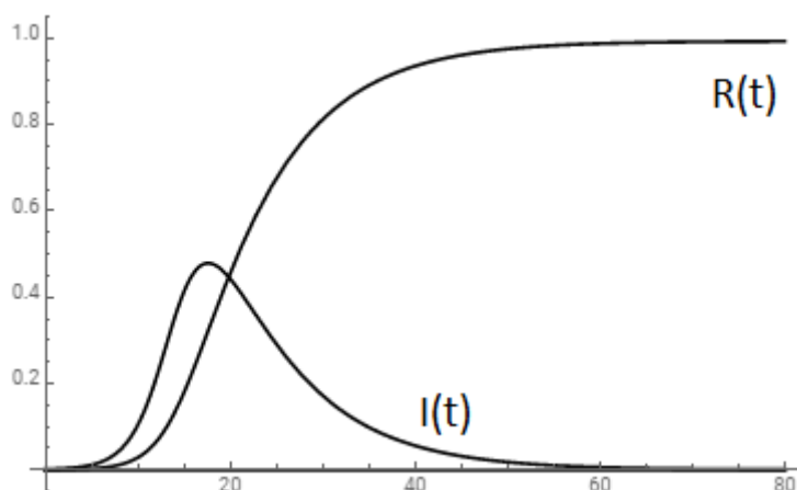
Fig.1. SIR model epidemic development ( \beta=0.6 , \gamma=0.12 )
