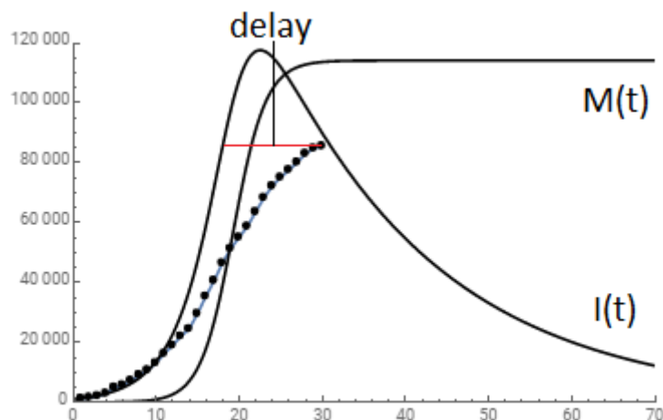
Fig. 5. Comparison of the dynamics of the number of cases during the COVID-19 epidemic in Spain according to the SIMR model (the solid line I(t) ) with statistical data [3] (the line with dots). The SIMR parameters are taken as m=0.39 , \beta=0.51 , \gamma=0.05 . Saturation of M(t) corresponds to 100% hidden immunization.
