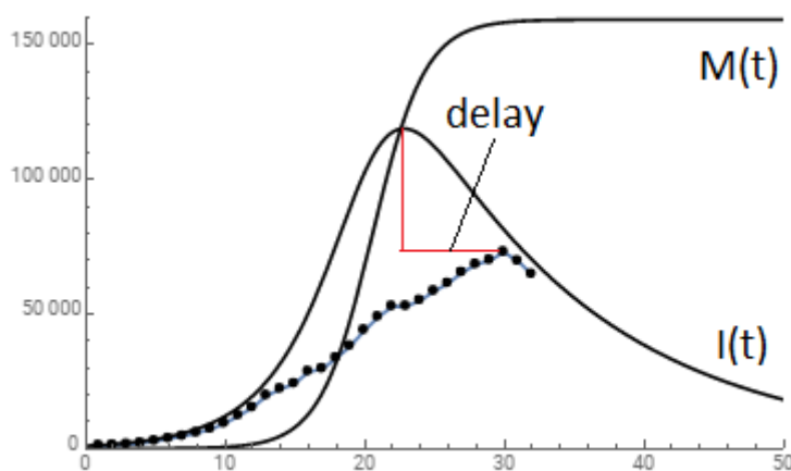
Fig. 6. Comparison of the dynamics of the number of cases during the COVID-19 epidemic in Germany according to the SIMR model (the solid line I(t) ) with statistical data [3] (the line with dots). The SIMR parameters are taken as m=0.39 , \beta=0.53 , \gamma=0.075 . Saturation of M(t) corresponds to 100% hidden immunization.
