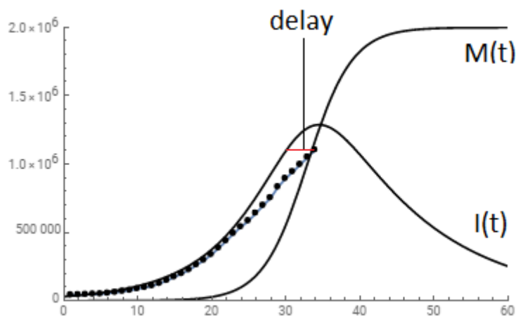
Fig. 10. Comparison of the dynamics of the number of cases during the COVID-19 epidemic in the World (without China) according to the SIMR model (the solid line I(t) ) with statistical data [3] (the line with dots). The SIMR parameters are taken as m=0.39 , \beta=0.33 , \gamma=0.075 . Saturation of M(t) corresponds to 100% hidden immunization.
