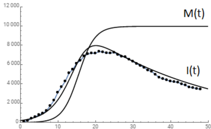
Fig. 9. Comparison of the dynamics of the number of cases during the COVID-19 epidemic in South Korea according to the SIMR model (the solid line I(t) ) with statistical data [3] (the line with dots). The SIMR parameters are taken as m=0.39 , \beta=0.46 , \gamma=0.03 . Saturation of M(t) corresponds to 100% hidden immunization. Fraction of the mutated virus in the total initial infection is taken to be f=0.9 .
