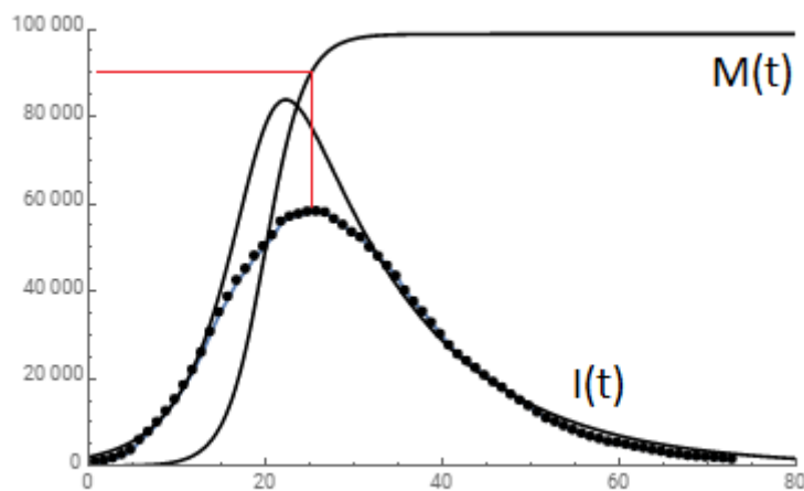
Fig. 3. Comparison of the dynamics of the number of cases during the COVID-19 epidemic in Wuhan (China) according to the SIMR model (solid line) with statistical data [3] (line with dots). The SIMR parameters are taken as m=0.39 , \beta=0.45 , \gamma=0.071 . Here and in all further figures, the line I(t) shows the number of cases, and the line M(t) is normalized to saturation with the value of M = 1 (100% hidden immunization). The red line indicates the hidden immunization M = 0.9 at the peak of I(t) .
