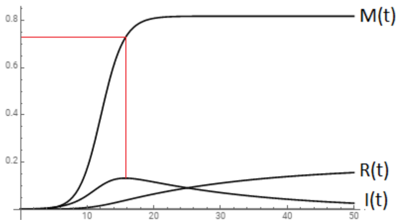
Fig. 2. SIMR epidemic development ( m = 0.2, \beta = 0.6, \gamma = 0.05 ). The red line indicates that at the peak of the epidemic, the percentage of hidden immunization M(t) is approximately 70%.
