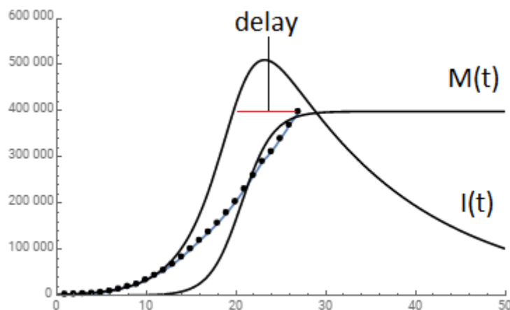
Fig. 8. Comparison of the dynamics of the number of cases during the COVID-19 epidemic in USA according to the SIMR model (the solid line I(t) ) with statistical data [3] (the line with dots). The SIMR parameters are taken as m=0.39 , \beta=0.57 , \gamma=0.065 . Saturation of M(t) corresponds to 100% hidden immunization.
