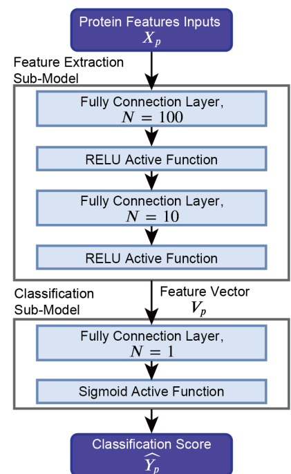
(b) DNN's structure diagram with optimal parameters
