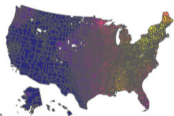
I Cluster 25
