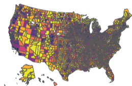
K Cluster 10
