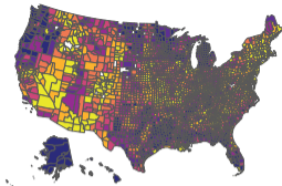
F Hydrazine
