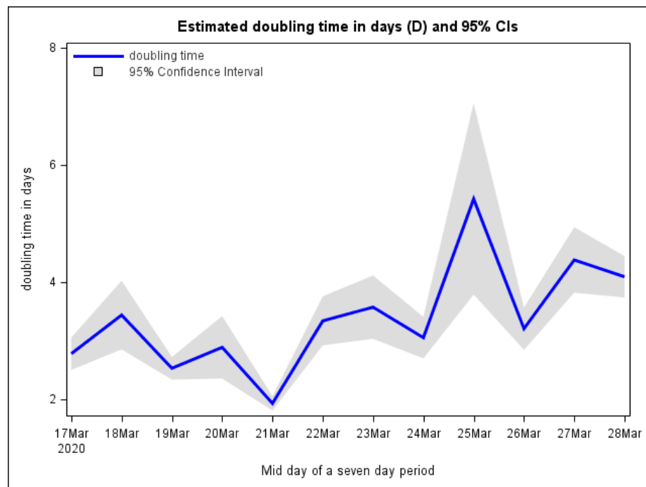
Figure 2. Estimated doubling time in days with 95% CIs over time using death data from New York State.
