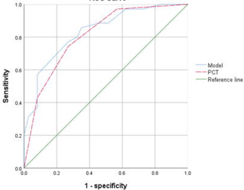
ROC Curve
