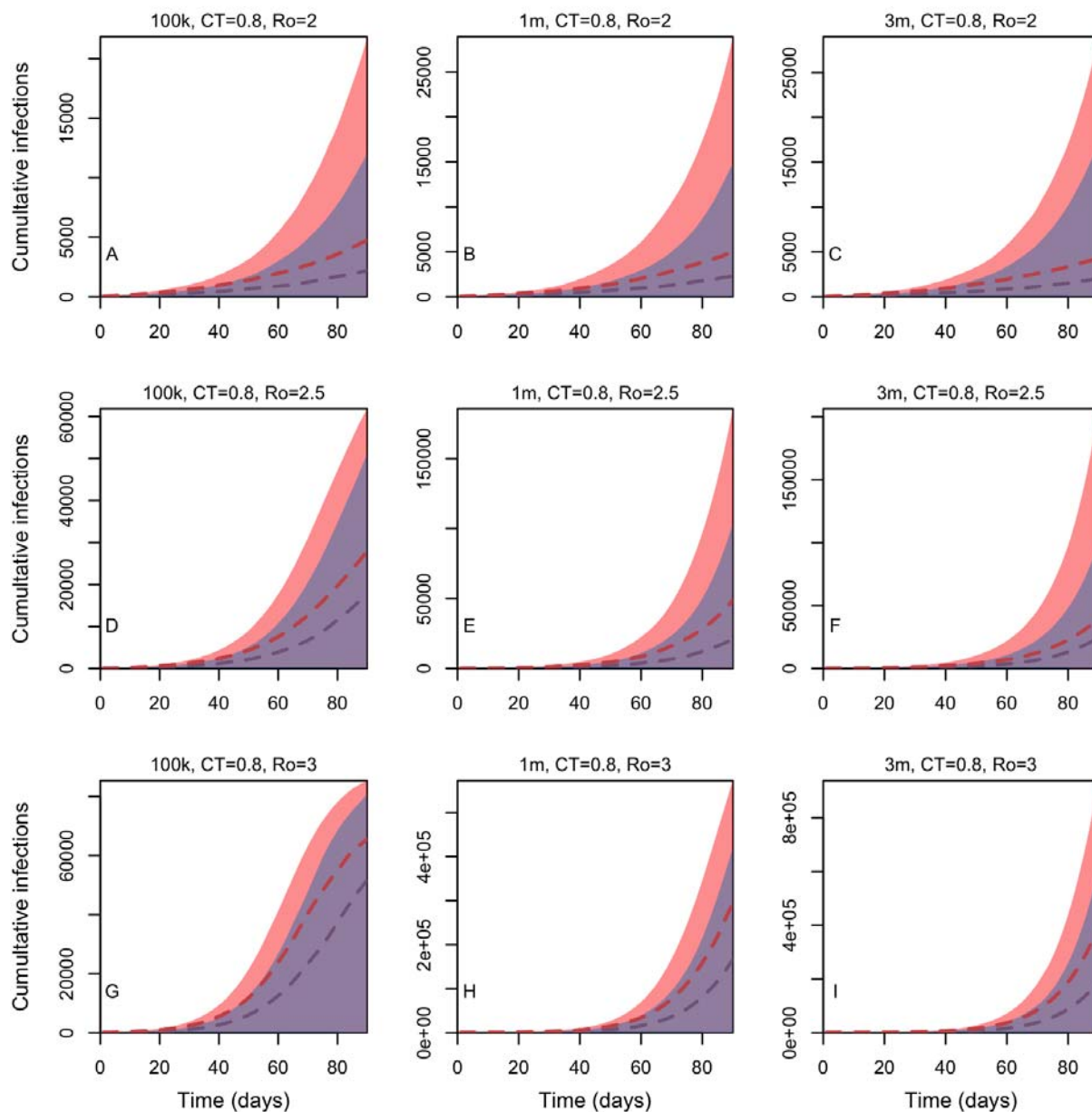
Fig 2: Cumulative number of infections in the initial 90 days with 50 (blue) and 100 (red) initial cases and 80% contact tracing, assuming R_0=2 , 2.5 and 3 (top to bottom respectively) for the three population sizes (left to right). Broken lines show the medians and corresponding regions show the 95% confidence interval.
