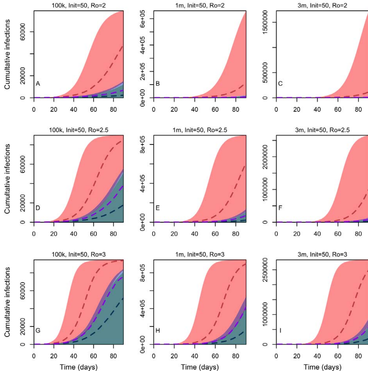
Fig 1: Cumulative number of infections in the initial 90 days with 0% (red), 50% (blue), and 80% contact tracing (green) and 50 initial cases, assuming R_0=2 , 2.5 and 3 (top to bottom respectively) for the three population sizes (left to right). Broken line shows the median value and corresponding regions show the 95% confidence interval.
